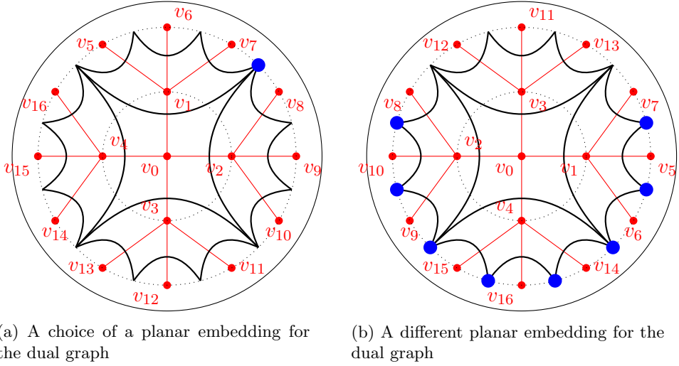
Figure 4. The region at the boundary of the dual graph “in between” boundary points v_8 and v_7 for two choices of planar embedding for the dual graph, depicted in blue.
