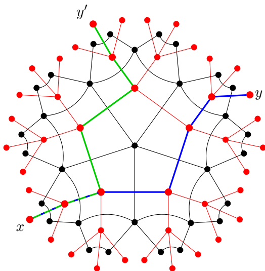
Figure 10. Geodesics in the BTZ black hole geometry. Moving y to y' leads to a “jump” of the minimal geodesic to a path wrapping the other side of the horizon.
