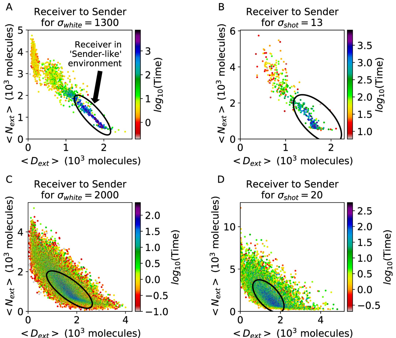
Fig 5. Timescales for single cell and lattice transitions. (a) The distribution of transition waiting times from Receiver to Sender as a function of N_{\text{EXT}} and D_{\text{EXT}} in a simulation starting from randomized initial conditions with white noise amplitude of \sigma_{\text{white}} = 1300 for 9000 hr after a 1000 hr relaxation period. Each dot represents the average switching event, while the x- and y-coordinates represent the average levels of Delta and Notch in neighboring cells during the transition. The color scale depicts the waiting time before the transition event. The "correct" state region (a Receiver surrounded by Sender-like environment) is circled, and dots within this region exhibit the longest transition waiting time. (b) Same as (a) but for \sigma_{\text{shot}} = 13 . (c) Same as (a) but at a high white noise level ( \sigma_{\text{white}} = 2000 ). These larger fluctuations also flip cells from the "correct" to "incorrect" state. (d) Same as (a) but for high shot noise ( \sigma_{\text{shot}} = 20 ).
