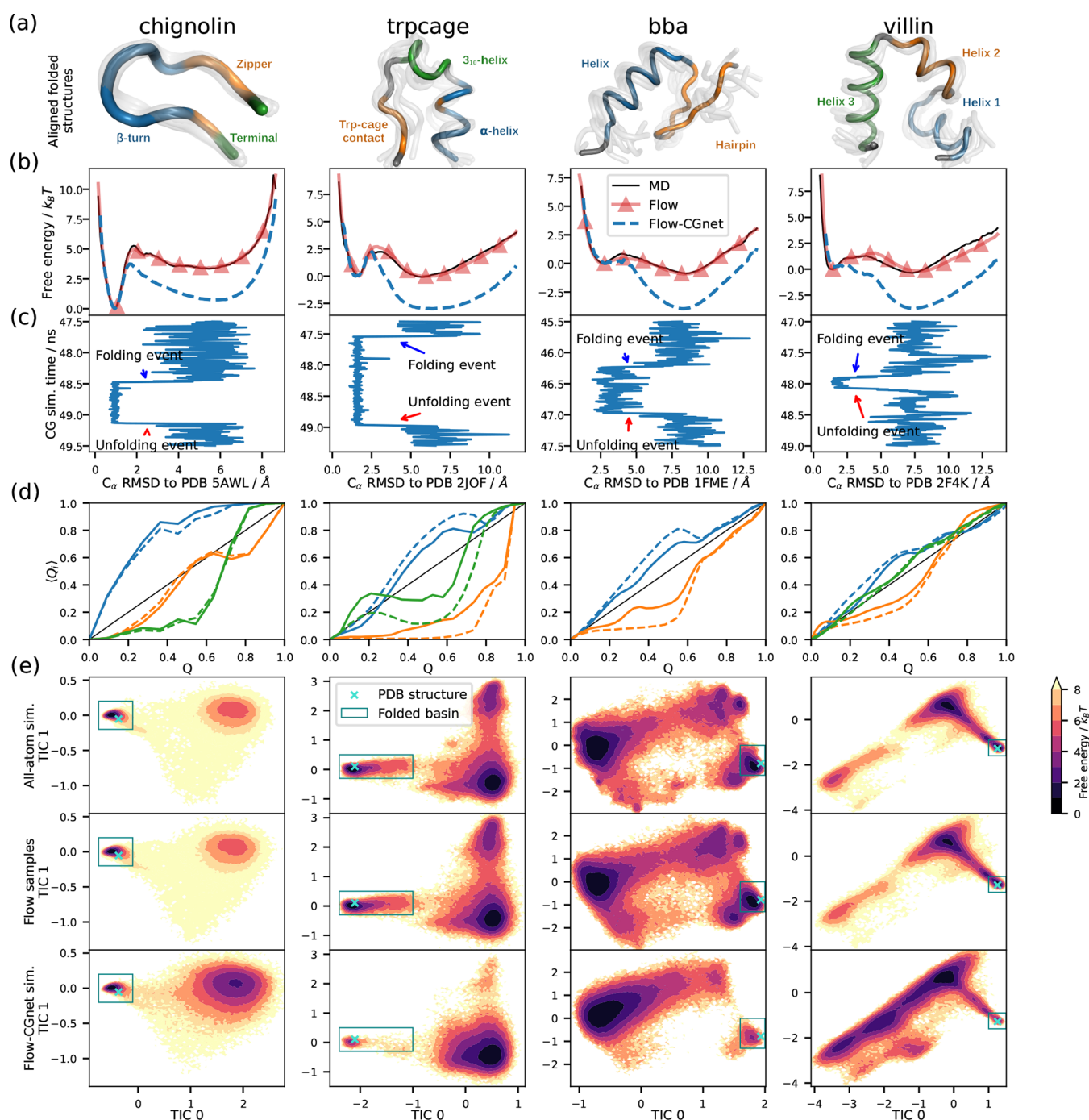
Figure 4. Flow-matching results for four fast-folding proteins. From top to bottom: (a) 10 exemplar folded samples from CG simulation (shown in half-transparent gray color) superposed on the experimental structure (colored segments correspond to important elements in the folding process); (b) free energy curve over RMSD for the MD, flow, and Flow-CGnet samples with PDB structure as the reference; (c) RMSD time series excerpted from CG simulation showing folding and unfolding events; (d) average fractions of native contacts ( Q_i ) in different segments of the protein formed at each stage of the folding process (identified by the fraction of all native contacts formed, Q ; segments are determined mainly according to secondary structures and are highlighted with the corresponding color in panel a); (e) free energy landscapes of all-atom MD, flow, and Flow-CGnet model over TICs (turquoise crosses and teal rectangles denoting experimental structures and folded state according to MD trajectories, respectively).
