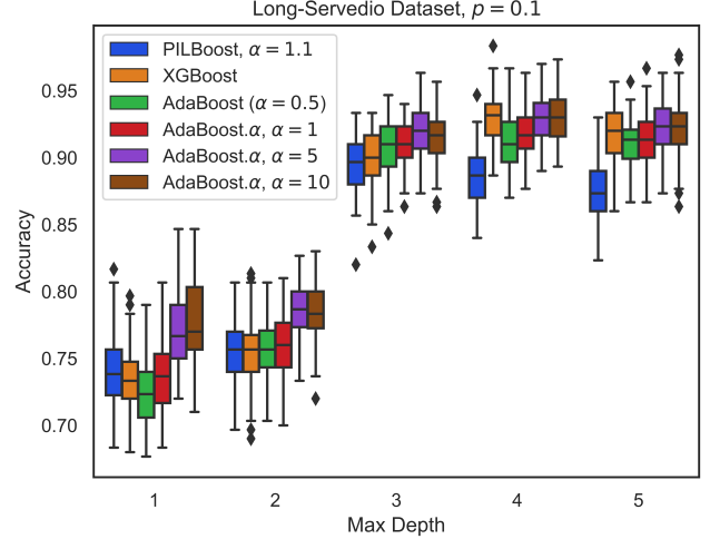
Figure 4: Box and whisker plots of the clean test accuracies of several boosters with 100 decision trees of varying maximum depth on the Long-Servedio dataset for p = 0.1 symmetric label noise. The boxes are the interquartile ranges, the lines in the boxes are the medians, and the diamonds are the outliers. Note that AdaBoost. \alpha with \alpha > 1 (quasi-convex), outperforms the convex boosters when the maximum depth is 1 or 2. Further commentary is in Section 5.1, and more noise levels are in Appendix B.1.
