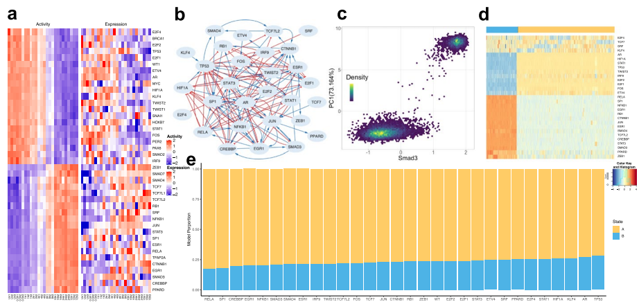
Fig. 5 Network modeling of TGF-β-induced EMT. Application of NetAct to an EMT in human cell lines using time-series microarray data. a Experimental expression and activity of enriched transcription factors. b Inferred TF regulatory network. Blue lines and arrowheads represent the gene activation; red lines and blunt heads represent gene inhibition. c The relationship between SMAD3 gene activity and the first principal component of the activity of all network genes from RACIPE simulations. d Hierarchical clustering analysis of simulated gene activity (with Pearson correlation as the distance function and Ward.D2 linkage method). Colors at the top indicate the two clusters from the simulated gene activity. The blue cluster represents the mesenchymal state, and the yellow cluster represents the epithelial state. The color legend for the heatmap is at the bottom right. e Knockdown simulations of the TF regulatory network. The bar plot shows the proportion of RACIPE models in each state (epithelial or mesenchymal) for the conditions of the knockdown of every TF
