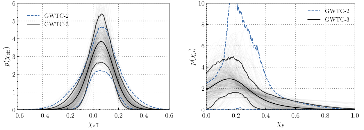
FIG. 16. Left panel: inferred distribution of \chi_{\text{eff}} for our latest full analysis in black. For comparison, the blue distribution and interval shows our inferences derived from GWTC2. Right panel: corresponding result for \chi_p . While both panels in this figure are derived using the Gaussian spin model, we find similar conclusions with the other spin models used to analyze GWTC-2.
