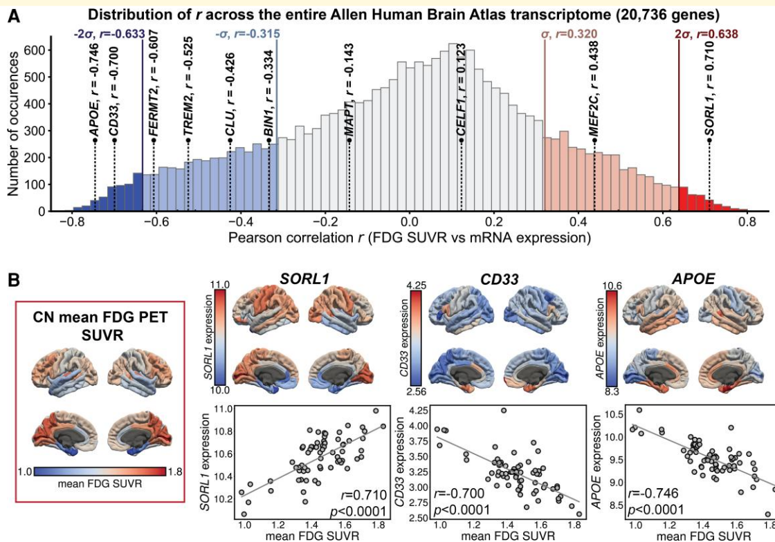
Figure 4 APOE, CD33 and SORL1 showed especially strong correlation with brain metabolism. (A) Distribution of 20 736 Pearson correlation coefficients, calculated between expression of 20 736 genes and mean FDG PET SUVR averaged across all CN participants. Light blue and red vertical lines represent z -score = -1 and 1 (i.e. one standard deviation away from mean), respectively. Vertical lines labelled with \sigma indicate the z -score = -1 and 1 (i.e. one standard deviation away from mean), respectively. Vertical lines labelled with 2\sigma indicate z -score = -2 and 2 . Bars in the distribution outside of the two standard deviations are coloured deep blue (negative correlations) and deep red (positive correlations), respectively. Bars in the distribution between one and two standard deviations are coloured light blue and light red, respectively. Using a z -score cut-off of \pm 2.0 , SORL1, CD33 and APOE showed strong correlation when compared with the distribution. (B) Left, in rectangular frame: mean FDG PET SUVR across all CN participants mapped to the 68 cortical ROIs. Right, top panel: expression of SORL1, CD33 and APOE, mapped to the 68 cortical ROIs, respectively. Right, bottom panel: scatter plots showing the correlation between mean FDG PET SUVR and gene expression of SORL1, CD33 and APOE, respectively. A linear fit is also provided in each scatter plot. FDG SUVR for each cohort and for each gender can be found in Supplementary Tables 16–19.
