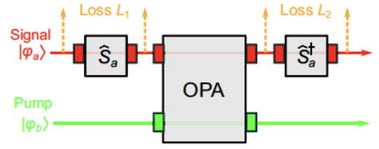
FIG. 5. The construction of an extended PNR QND measurement. The external squeezing operations modify the measured observable to \hat{N}_{\text{eff}} = \hat{S}_a^\dagger \hat{N}_a \hat{S}_a . We model the loss of each squeezer by a pair of equal beam splitters placed before and after the squeezer.
