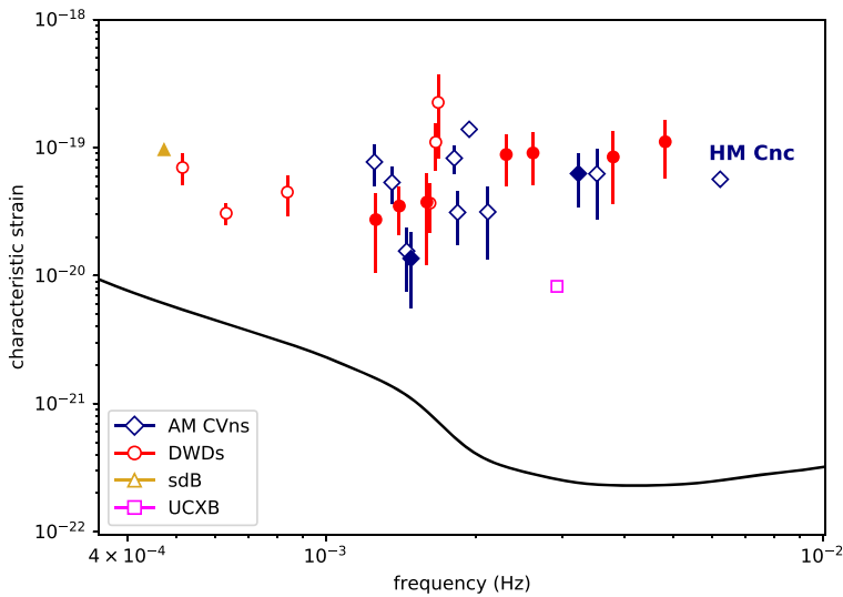
Fig. 2 Sensitivity plot for LISA assuming 10 year of observation with an 80% duty cycle showing the known binaries which reach a \text{SNR} \geq 5 . Filled symbols represent eclipsing sources and open symbols represent non-eclipsing sources from Kupfer et al. (2018). The black lack solid line represents the LISA sensitivity curve. Acronyms for binaries: AM Canum Venaticorum (AM CVns), WD+WD (DWDs), subdwarf B-star (sdB) and ultracompact X-ray binary (UCXB). Image credit: Thomas Kupfer
