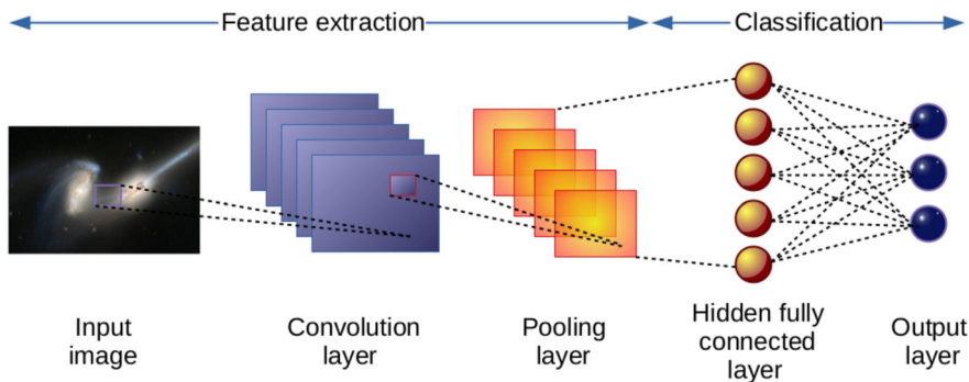
Fig. 28 Schematic representation of a basic convolutional neural network architecture. Such numerical network can be trained on simulations, and later apply to observations to systematically identify MBHB candidates. Image credit: Ioana Dutan
