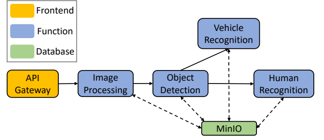
Figure 6: ML pipeline architecture.
