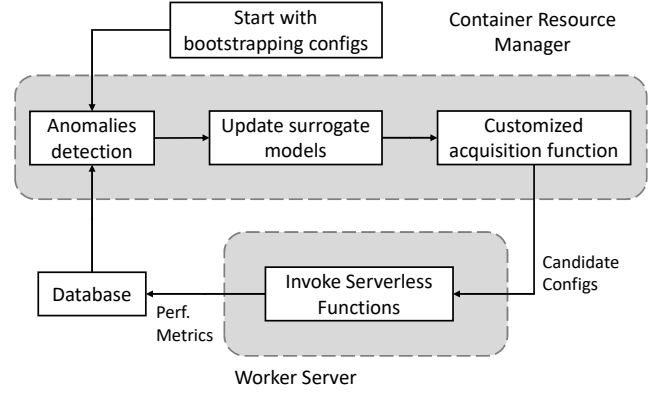
Figure 4: Workflow of Aquatope’s container resource manager.
