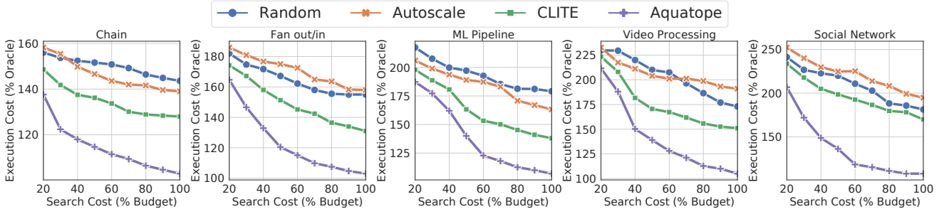
Figure 12: Iteratively searching for a near-optimal configuration across two synthetic and the three end-to-end workflows.
