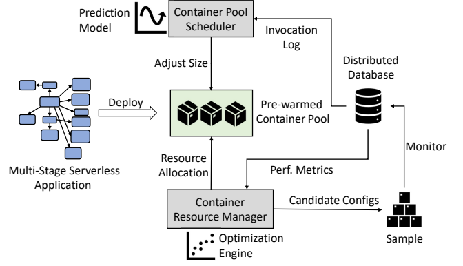
Figure 1: System overview of Aquatope.
