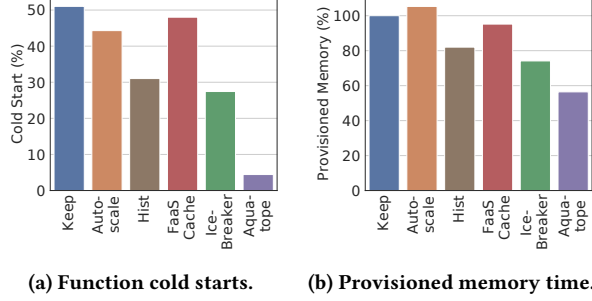
Figure 9: Aquatope’s dynamic pre-warmed container pool outperforms other empirical and data-driven approaches.
