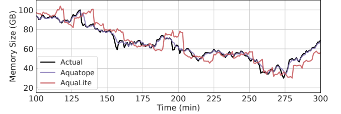
Figure 11: Aquatope’s dynamic pre-warmed container pool adapts to fluctuating workload better than the AquaLite that does not account for uncertainty.
