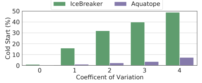
Figure 10: Aquatope outperforms IceBreaker, the best-performing previous work for cold start elimination, for input workloads with different coefficients of variation (CV). A CV greater than 1 suggests a large variation in the inter-arrival time of workflow invocations. Aquatope achieves higher benefits for highly fluctuating loads because it accounts for noise and uncertainty.
