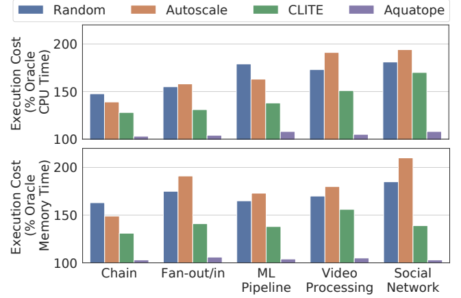
Figure 13: Aquatope’s resource manager finds a near-optimal resource configuration across multi-stage serverless applications.
