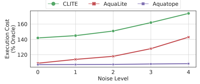
Figure 15: Aquatope’s robustness to cloud noise.
