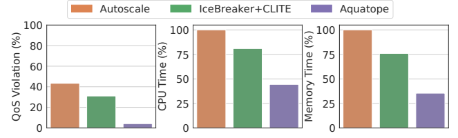
Figure 18: End-to-end performance analysis for Aquatope compared to autoscaling policies and a combination of the best prior work.
