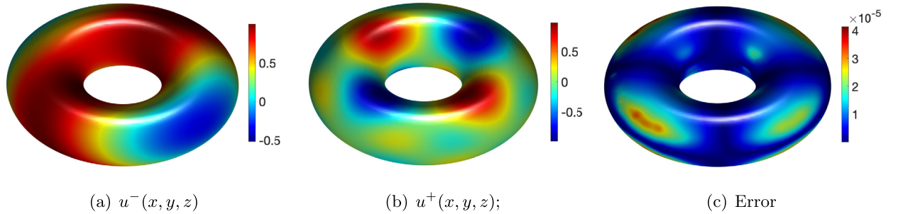
Fig. 13. The plots of exact solutions and numerical error of the ray-casting AMIB scheme by mapping onto the torus surface \Gamma , based on a mesh with n = 128 .
