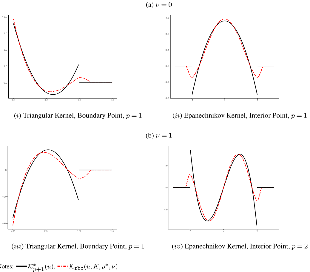
Figure 1: \mathcal{K}_{p+1}^*(u) vs. \mathcal{K}_{\text{rbc}}(u; K, \rho^*, \nu)
