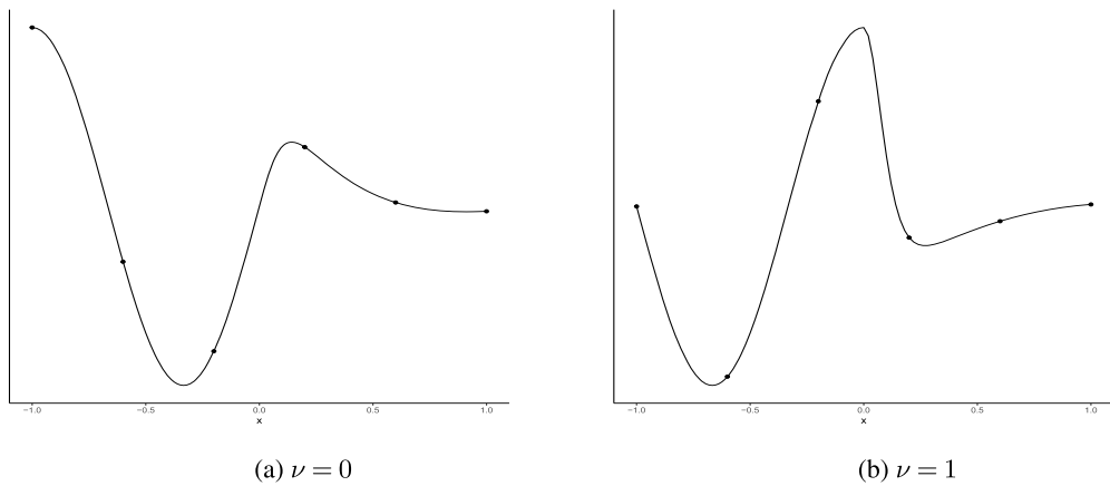
Figure 2: Conditional mean function and first derivative, \mu^{(\nu)}(x)
