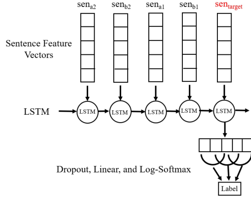
Fig. 5. The LSTM classifies the sentence with the dependence information from neighbor sentences.
