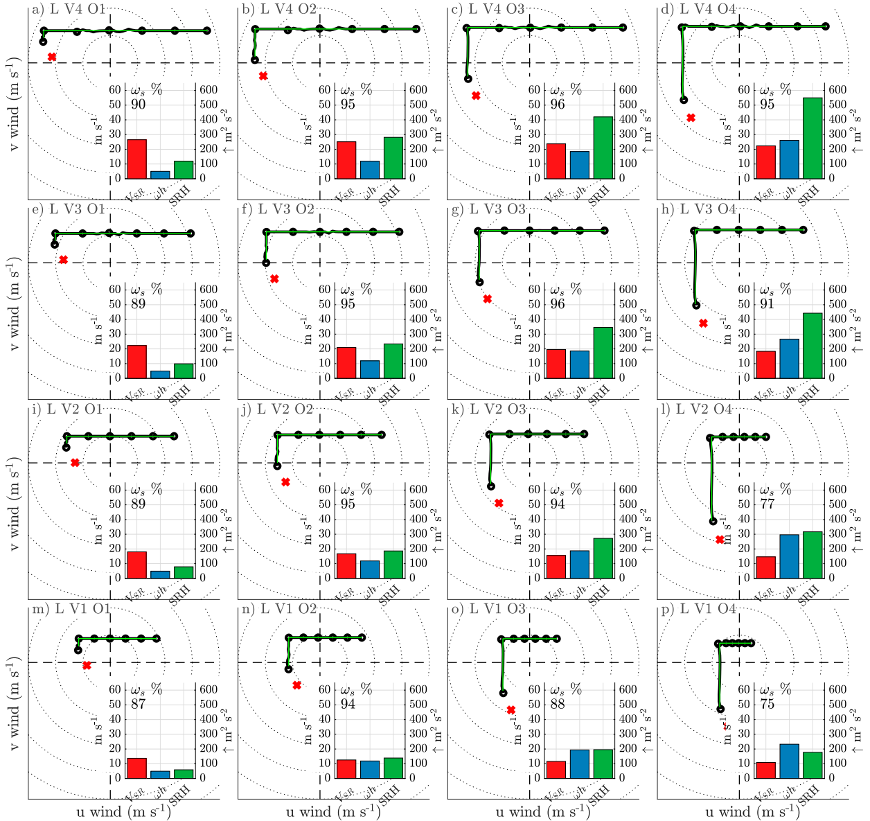
FIG. 2. Storm-relative hodographs for the 16 L simulations before (thin green lines) and after (thick black lines) the 15-h “spinup” period, with u and v wind on the x and y axes, respectively ( \text{m s}^{-1} ), and the origin representing the “Bunkers”-estimated right-mover storm motion. Dots are plotted on the hodograph curve from the surface to 6000 m AGL at intervals of 1000 m. Wind speed range rings are included every 10 \text{ m s}^{-1} . \omega_s increases from the leftmost column to the rightmost column, and V_{\text{SR}} increases from the bottom row to the top row. The red \times denotes the location where the ground-relative wind is zero. Each panel contains a subpanel in the lower right showing V_{\text{SR}} (red; \text{m s}^{-1} ), \omega_s h (i.e., streamwise vorticity times h , blue, \text{m s}^{-1} ), and SRH (green, \text{m}^2 \text{ s}^{-2} ). The quantities in the subpanel were computed using the adjusted profiles (i.e., after the 15-h spinup period). The horizontal streamwise vorticity percentage, defined as the layer average of the horizontal streamwise vorticity magnitude divided by the total horizontal vorticity magnitude, is listed in each subpanel.
