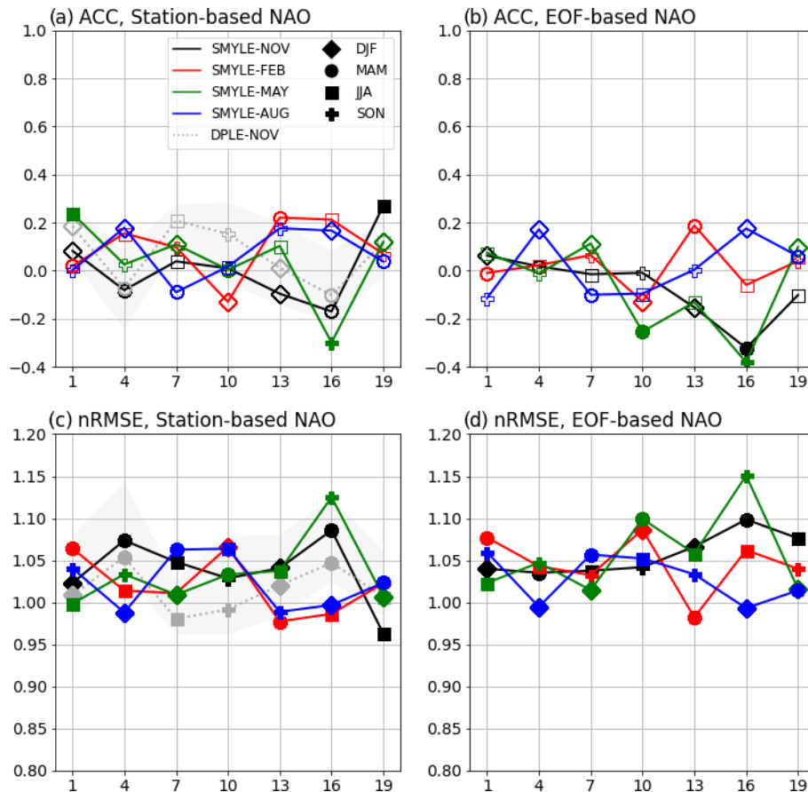
Figure 7. Anomaly correlation coefficient (ACC; a , b ) and nRMSE ( c , d ) for NAO as a function of initialization month and target season. Results are shown for both station-based ( a , c ; computed as the normalized SLP difference between model grid cells nearest to Lisbon, Portugal and Reykjavik, Iceland) and EOF-based ( b , d ; computed as the PC time series of the first EOF of SLP in the domain 20–80° N, 90° W–40° E) seasonal NAO. Filled symbols in panels ( a ) and ( b ) indicate significant ACC scores ( p < 0.1 ). Scores from 40-member DPLE-NOV are shown in dashed grey, with grey shading giving the 90 % confidence bounds obtained from 100 resamplings (across members) of 20-member DPLE-NOV. The verification dataset is ERA5.
