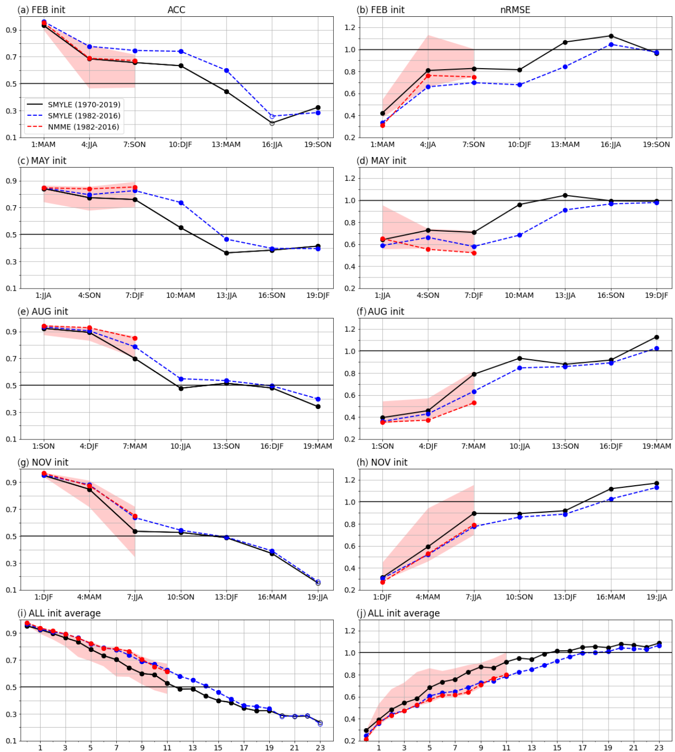
Figure 3. Anomaly correlation coefficient (ACC) on the left and normalized RMSE skill scores on the right for Niño-3.4 SST (regional average over 5^{\circ}\text{S} – 5^{\circ}\text{N} , 170 – 120^{\circ}\text{W} ). Panels (a)–(h) show skill for seasonal mean Niño 3.4 for 4 different start months (FEB, MAY, AUG, NOV), with the x axis showing lead time in months and target season. Panels (i) and (j) show skill for monthly mean Niño 3.4 averaged across all 4 start months as a function of lead time in months. Filled symbols for ACC (left panels) indicate significant correlation scores ( p < 0.1 ). SMYLE skill is shown for two different forecast sets: the full set initialized 1970–2019 (solid black curve) and a subset initialized 1982–2016 (dashed blue curve). The latter can be directly compared to NMME results, which are shown as scores for the full multi-model ensemble mean (dashed red curve) as well as the range of scores from eight individual NMME models (red shading). The verification dataset is HadISST1.
