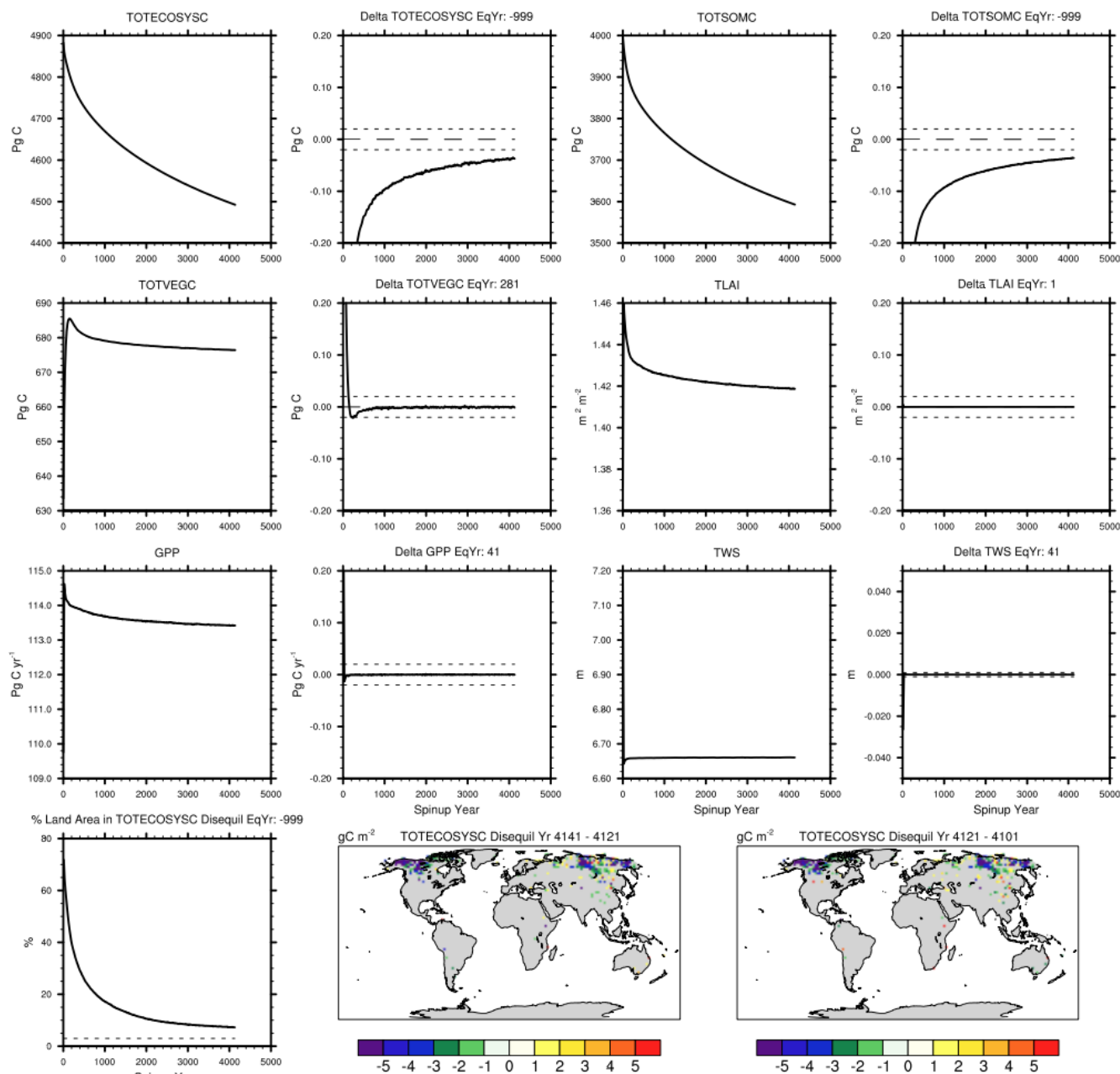
Figure A1. Evolution of land carbon fields in land-only spin-up simulation: total ecosystem carbon (TOTESYSC), total soil organic matter carbon (TOTSOMC), total vegetation carbon (TOTVEGC), total leaf area index (TLAI), gross primary productivity (GPP), and terrestrial water storage (TWS). Fields are plotted both as raw global average time series as well as “delta” time series that show the running difference between consecutive 20-year averages. The latter show that TOTSOMC dominates TOTESYSC and is the slowest term to equilibrate but has reached a reasonable delta value of around -0.04 Pg C after 4000 years of spin-up. The plots in the bottom row show that less than 10 % of global land area remains outside of the target delta range for TOTESYSC (shown as dashed lines in the delta plots) and that the regions associated with slight disequilibrium at the end of spin-up are concentrated in northern Siberia.
