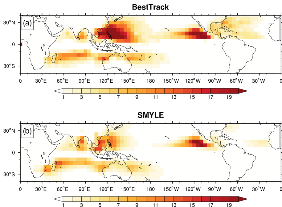
Figure B8. Annual mean global TC track density (over 5^\circ \times 5^\circ box) during 1970–2018 in (a) observations and (b) SMYLE lead month 1 forecasts (averaged over four initialization times).
