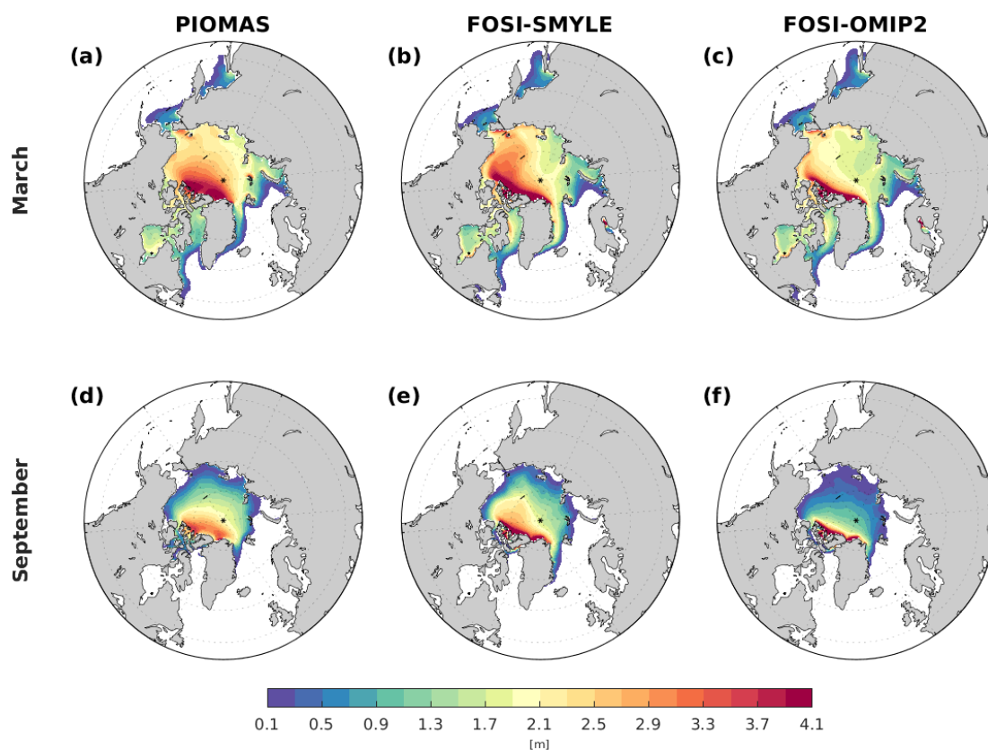
Figure A3. Climatological (1991–2010) sea ice thickness for March (a, b, c) and September (d, e, f) from (a, d) PIOMAS, (b, e) FOSI-SMYLE, and (c, f) FOSI-OMIP2.
