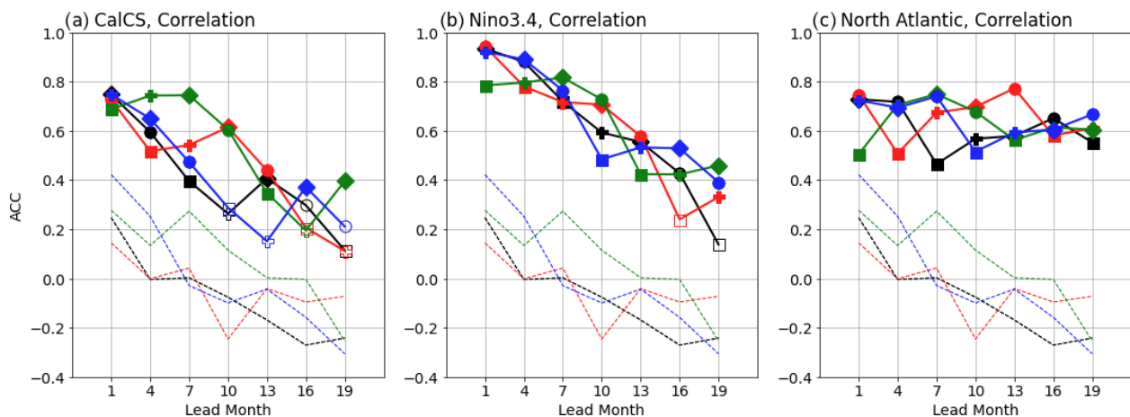
Figure 9. Anomaly correlation coefficients for aragonite saturation state ( \Omega_{\text{arag}} ) averaged over (a) the California Current System LME, (b) the Niño-3.4 region, and (c) the subpolar North Atlantic (55–60° N, 30–50° W). Colored solid lines and symbols denote SMYLE initializations and verification seasons, respectively. Colored dashed lines give persistence forecast results for different initialization months. Filled symbols in panels (a)–(c) indicate significant ACC scores ( p < 0.1 ).
