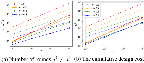
Figure 4: Boundary design on RPS. The dashed lines are the theoretical upper bound.
