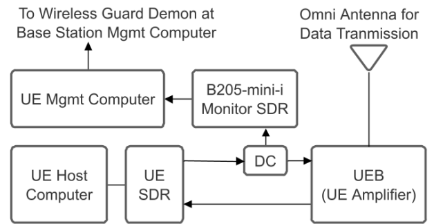
Figure 5: Wireless Guard Hardware Architecture for UE Node
