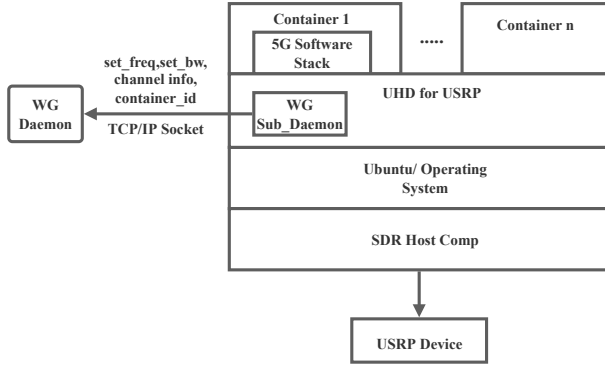
Figure 6: Architecture for Proactive Approach
