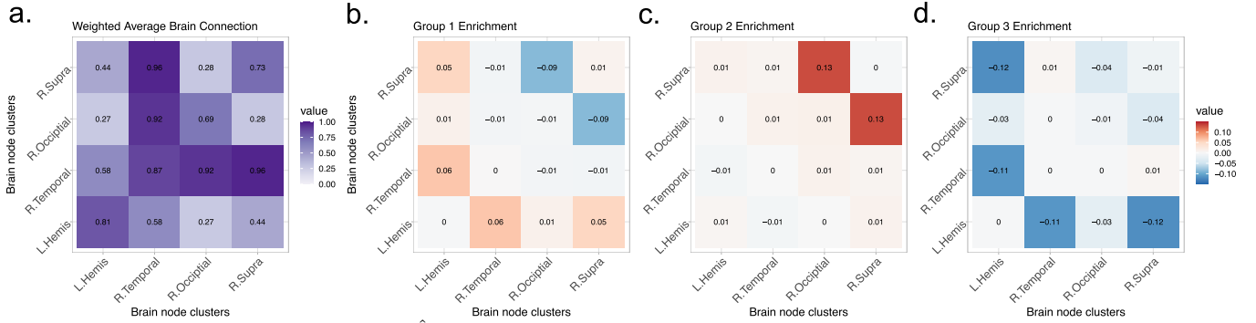
Fig. 10. Mode 3 slices of estimated core tensor \hat{\mathcal{S}} . (a) Average estimated slice weighted by the group size; (b)-(d) Group-specified enrichment, i.e., the difference between each slice of \hat{\mathcal{S}} and the averaged slice.
