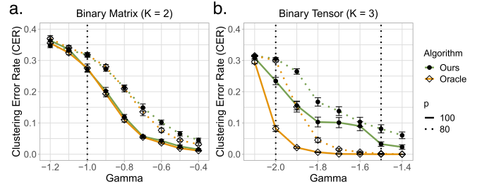
Fig. 12. SNR phase transitions for Bernoulli dTBM with p = \{80, 100\}, r = 5 under (a) matrix case with \gamma \in [-1.2, -0.4] and (b) tensor case with \gamma \in [-2.1, -1.4] .
