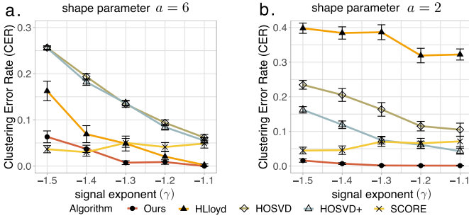
Fig. 7. CER comparison versus signal exponent (denoted \gamma ) under (a) low (shape parameter a = 6 ) (b) high (shape parameter a = 2 ) degree heterogeneity. We set p = 100, r = 5, \gamma \in [-1.5, -1.1] under Gaussian model.
