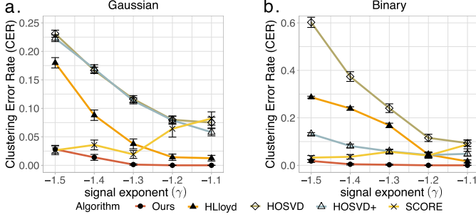
Fig. 6. CER versus signal exponent (denoted \gamma ) for different methods. We set p = 100, r = 5, \gamma \in [-1.5, -1.1] under (a) Gaussian and (b) Bernoulli models.
