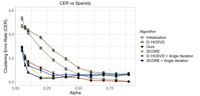
Fig. 13. CER comparison versus sparsity parameter \alpha_p in [0.05, 0.9] . We set p = 100, r = 5 and \gamma = -1.2 under sparse binary dTBM.
