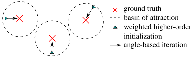
Fig. 3. Illustration of our global-to-local algorithm.
