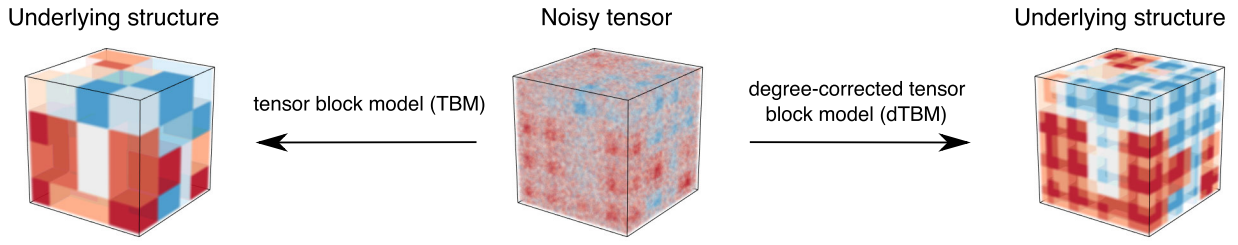
Fig. 1. Examples for order-3 tensor block model (TBM) with and without degree correction. Both TBM and dTBM have four communities on each mode, while dTBM allows a richer structure with degree heterogeneity.
