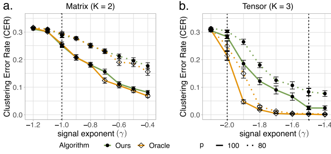
Fig. 4. SNR phase transitions for clustering in dTBM with p = \{80, 100\} , r = 5 under (a) matrix case with \gamma \in [-1.2, -0.4] and (b) tensor case with \gamma \in [-2.1, -1.4] .
