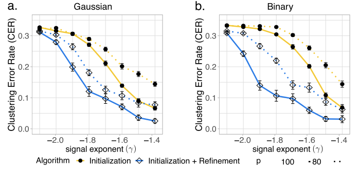
Fig. 5. CER versus signal exponent ( \gamma ) for initialization only and for combined algorithm. We set p = \{80, 100\} , r = 5 , \gamma \in [-2.1, -1.4] under (a) Gaussian models and (b) Bernoulli models.
