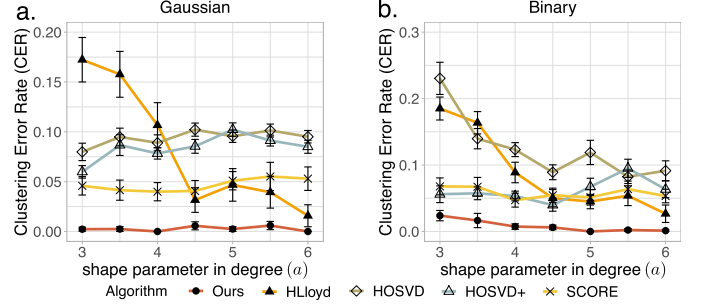
Fig. 8. CER versus shape parameter in degree (denoted a \in [3, 6] ) for different methods. We set p = 100, r = 5, \gamma = -1.2 under (a) Gaussian and (b) Bernoulli models.
