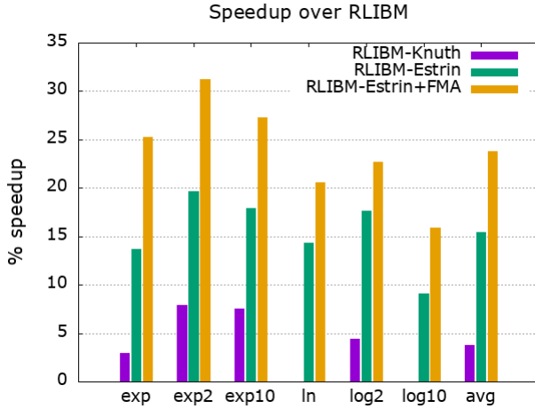
Figure 6. Speedup of the polynomial approximations generated by RLIBM-Knuth, RLIBM-Estrin, and RLIBM-Estrin+FMA methods in comparison to functions in the RLIBM project.
