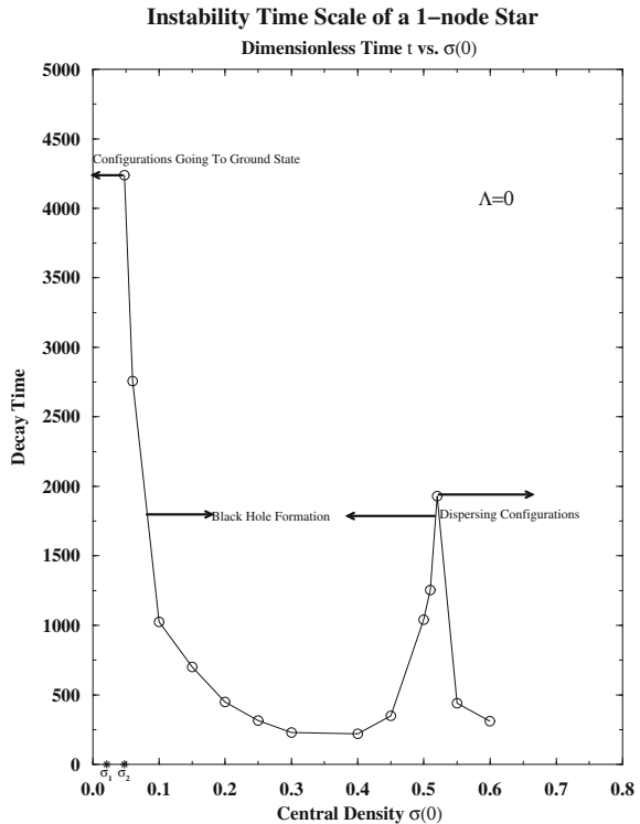
Fig. 16 The instability time scale of an excited boson star (the first excitation) to one of three end states: (i) decay to the ground state, (ii) collapse to a black hole, or (iii) dispersal. Reproduced with permission from Balakrishna et al. (1998), copyright by APS
