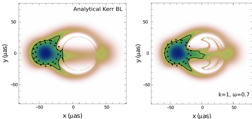
Fig. 30 Computed images as might be expected from the EHT for: (left) a Kerr black hole and (right) a fast spinning boson star with accretion according to certain assumptions. The similarity in images indicates that ruling out a BS candidate in images of Sgr A* may prove difficult.
