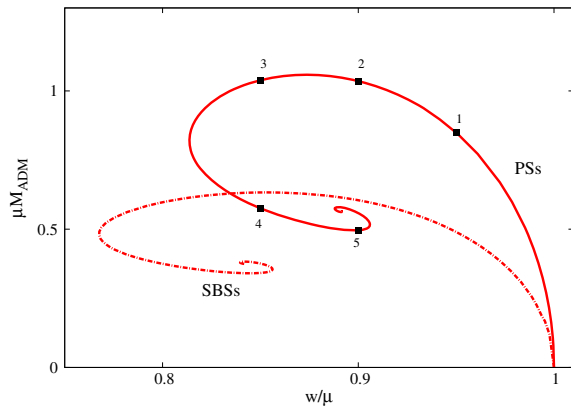
Fig. 13 Comparison of Proca solutions with boson stars. The ADM mass of spherical Proca solutions (solid) and scalar BS solutions (dashed) are shown versus oscillation frequency. Here, the mass is expressed in terms of the field mass, \mu . Although the profiles are qualitatively similar, notice that the maximum mass of the Proca solutions is almost twice that of BSs. Reproduced with permission from Sanchis-Gual et al. (2017b), copyright by APS
