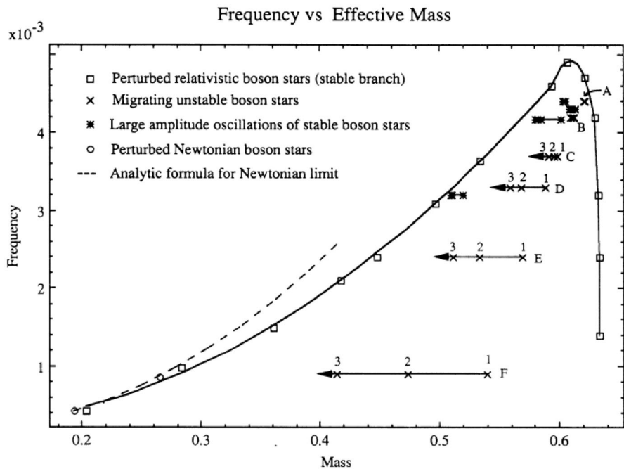
Fig. 15 Oscillation frequencies of various boson stars are plotted against their mass. Also shown are the oscillation frequencies of unstable BSs obtained from the fully nonlinear evolution of the dynamical system. Unstable BSs are observed maintaining a constant frequency as they approach a stable star configuration.
