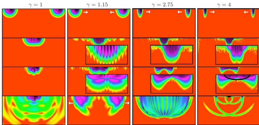
Fig. 35 Evolutions of the head-on collisions of identical boson stars boosted toward each other with initial Lorentz factors \gamma as indicated. Time flows downward within each column and the top edge displays the axis of symmetry. The color-scale indicates the value of |\phi| . In the middle frames one sees the interference pattern characteristic of high kinetic energy BS collisions (as mentioned in Fig. 1). In the last column on the right, the collision produces a BH with apparent horizon indicated by the black oval in the third frame. Reproduced with permission from Choptuik and Pretorius (2010), copyright by APS
