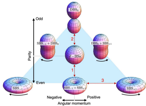
Fig. 12 The energy density distribution of the different k = 1 hybrid- \ell -boson stars. In this case, we see: dipole BSs (DBS 0 ), spinning BSs, (SBS ±1 ), spinning dipolar BSs (DBS 0 + SBS ±1 ), toroidal static BSs (SBS -1 + SBS +1 ), and finally \ell -BSs (SBS -1 + DBS 0 + SBS +1 ). Reproduced with permission from Sanchis-Gual et al. (2021), copyright by APS
