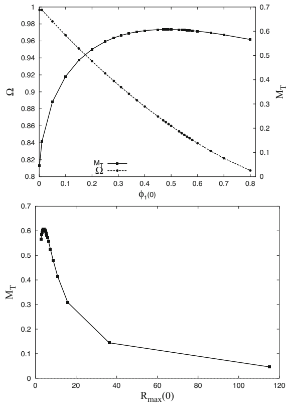
Fig. 6 Top : Total mass (in units of M_{\text{Planck}}^2/m ) and fundamental frequency of an oscillaton as a function of the central value of the scalar field \phi_1(r=0) . The maximum mass is M_{\text{max}} = 0.607 M_{\text{Planck}}^2/m . Bottom : Plot of the total mass versus the radius at which g_{rr} achieves its maximum. Reproduced with permission from Alcubierre et al. (2003); copyright by IOP
