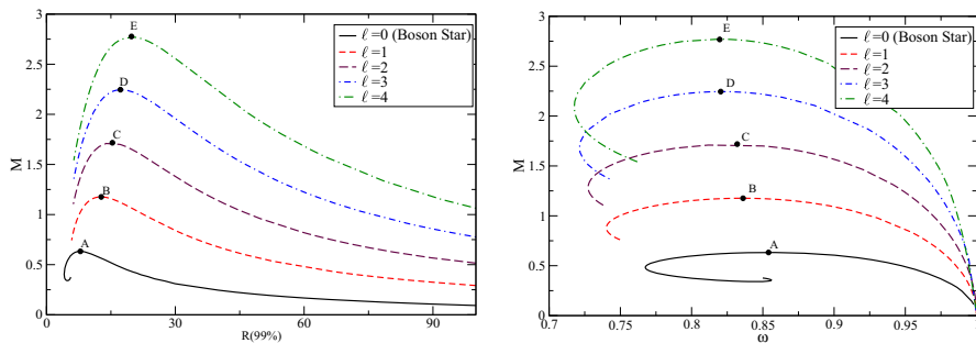
Fig. 11 \ell -boson stars: (Left) Total mass as a function of the effective radius for equilibrium configurations of different angular momentum number, denoted here as \ell . Note that the mass increases more quickly with k than the radius, and hence the compactness increases. (Right) Total mass as a function of the frequency of oscillation for the same configurations as in the left panel.
