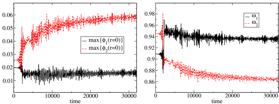
Fig. 10 Left: The maximum of the central value of each of the two scalar fields constituting the multi-state BS for the fraction \eta = 3 , where \eta \equiv N^{(2)}/N^{(1)} defines the relative “amount” of each state. Right: The frequencies associated with each of the two states of the multi-state BS. At t = 2000 , there is a flip in which the excited state (black solid) decays and the scalar field in the ground state (red dashed) becomes excited. Discussed in Sect. 3.7.
