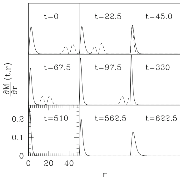
Fig. 34 Evolution of a boson star (solid line) perturbed by a shell of scalar field (dashed line). Shown is the mass density \partial M / \partial r for each contribution. By t \approx 100 the real scalar field pulse has departed the central region and perturbed the boson star into an unstable, compact configuration. Contrast the t = 0 frame with that of t = 97.5 and note the increase in compaction. This unstable BS survives until t \approx 500 only because the initial perturbation has been tuned to one part in 10^{15} and indicates Type I critical behavior. Reproduced with permission from Lai and Choptuik (2007)
