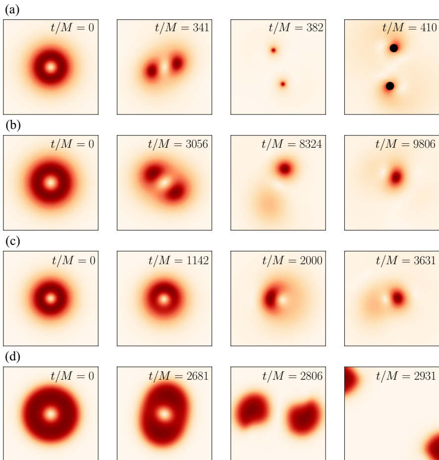
Fig. 20 Series of snapshots showing the evolution of |\phi|^2 in four scenarios where an unstable rotating BS with k = 1 undergoes the NAI reaching different end states. From top to bottom: a a mini-BS that collapses to a binary BH (the regions inside the apparent horizons are indicated in black), b a rotating mini-BS resulting in a non-rotating with non-negligible linear momentum, c a BS with strong self-interaction yielding a non-rotating BS with large linear momentum, and d an axion BS where the NAI results in the fragmentation of the star into two equal-mass non-rotating BSs.
