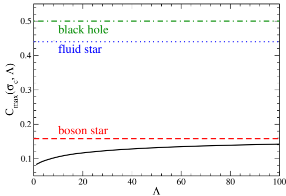
Fig. 4 The compactness of a stable boson star (black solid line) as a function of the adimensional self-interaction parameter \Lambda \equiv \lambda/(4\pi Gm^2) . The compactness is shown for the most massive stable star (the most compact BS is unstable). This compactness asymptotes for \Lambda \rightarrow \infty to the value indicated by the red, dashed line. Also shown for comparison is the compactness of a Schwarzschild BH (green dot-dashed line), and the maximum compactness of a non-spinning neutron star (blue dotted line). Reproduced with permission from Amaro-Seoane et al. (2010), copyright by IOP
