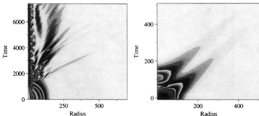
Fig. 18 The evolution of r^2\rho (where \rho is the energy density of the complex scalar field) with massive field (left) and massless (right). In the massive case, much of the scalar field collapses and a perturbed boson star is formed at the center, settling down by gravitational cooling. In the massless case, the scalar field bounces through the origin and then disperses without forming any compact object.
