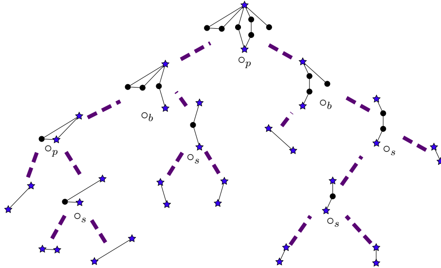
Figure 8: A GSP decomposition T . The starred vertices are terminals of their respective graphs. Each node \mathbf{H} is labelled with \circ_{T,\mathbf{H}} .
