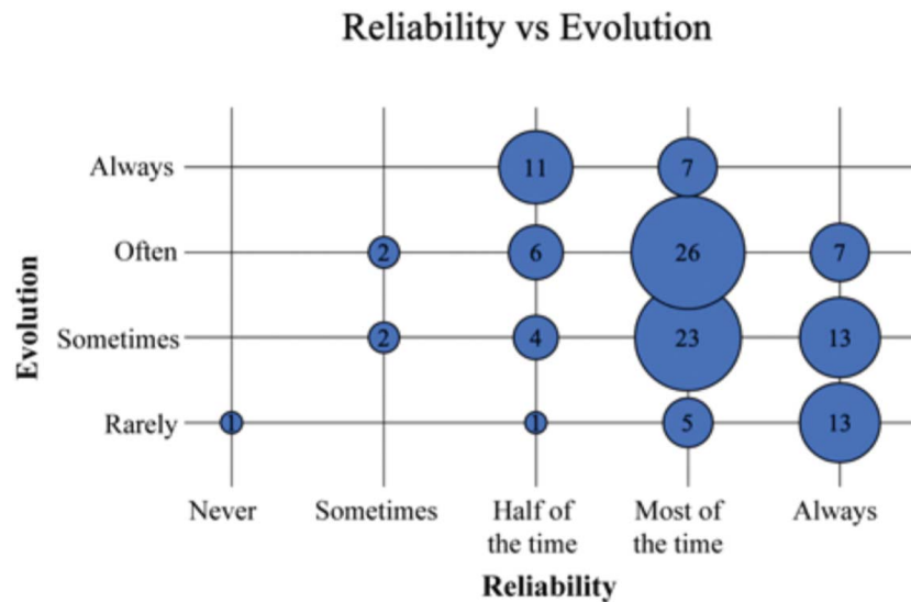
Fig. 15 Combination of responses for heuristic reliability versus its evolution (N = 121)
