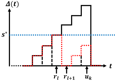
Fig. 11: An illustration of the advantage of a constructed capped reactive policy \pi' \in \Pi^{R+} over an arbitrary given non-capped reactive policy \pi \in \Pi^R \setminus \Pi^{R+} , where the solid black curve and the dashed red curve denote the AoI trajectories under policies \pi and \pi' , respectively.
