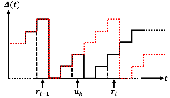
Fig. 10: An illustration of the advantage of a constructed reactive policy \pi' \in \Pi^R over an arbitrary given non-reactive policy \pi \in \Pi \setminus \Pi^R , where the solid black curve and the dashed red curve denote the AoI trajectories under policies \pi and \pi' , respectively.
