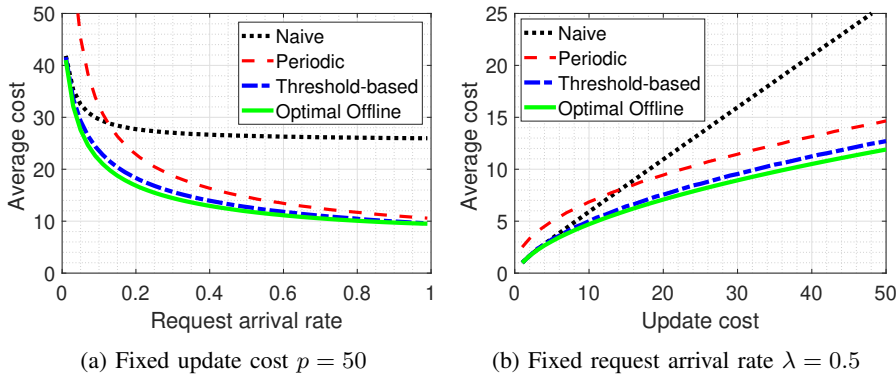
Fig. 6: Performance comparisons of different policies with different request arrival rate \lambda and different update cost p when f(\Delta) = \Delta , respectively.
