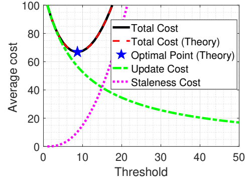
Fig. 5: Average cost under threshold-based policies with different thresholds when f(\Delta) = \Delta^2 , where \lambda = 0.1 and p = 100 .
