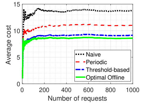
Fig. 7: Performance comparisons of different policies using trace dataset, where update cost p = 25 , request arrival rate \lambda = 0.4 , and f(\Delta) = \Delta .
