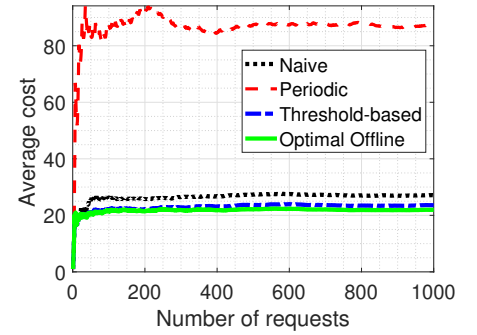
Fig. 9: Performance comparisons of different policies using trace dataset, where update cost p = 50 , request arrival rate \lambda = 0.4 , and f(\Delta) = \Delta^2 .
