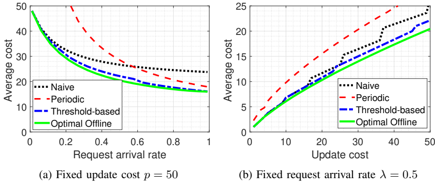
Fig. 8: Performance comparisons of different policies with different request arrival rate \lambda and different update cost p when f(\Delta) = \Delta^2 , respectively.
