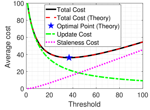
Fig. 4: Average cost under threshold-based policies with different thresholds when f(\Delta) = \Delta , where \lambda = 0.1 and p = 100 .
