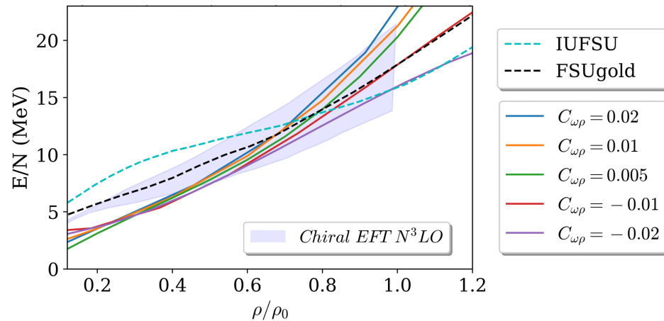
Figure 2. Energy per nucleon of pure neutron matter as a function of density for 5 different parameter sets. The shaded area corresponds to Chiral EFT constraints as provided in Ref. [22]. The RMF models FSUgold and IUFSU, which also include the \omega - \rho interaction, are shown for comparison. Note that here the saturation density \rho_0 = 0.165 \text{ fm}^{-3} .
