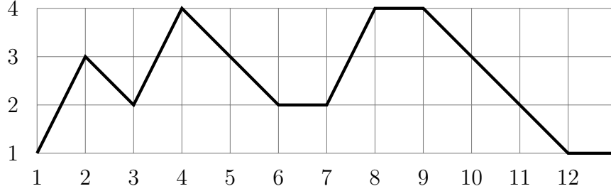
Figure 12: A periodic generalized Motzkin path of length \mathbf{n} = 12 corresponding to the (1, 3) -composition 1, 1, 0, 1; 1, 1, 2 , starting with an up step from the first floor.
