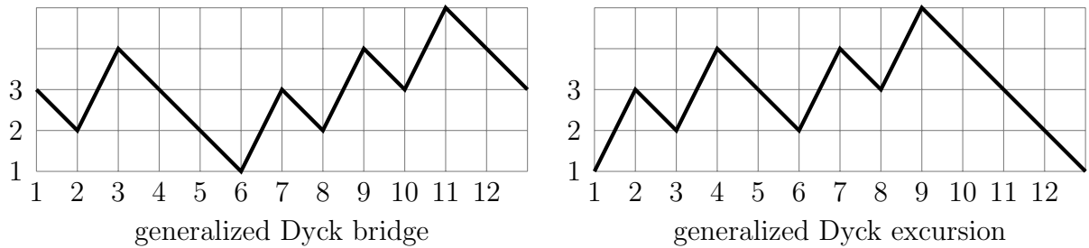
Figure 1: A generalized Dyck bridge and a generalized Dyck excursion for g = 3 , which starts from the first floor, of length \mathbf{n} = 12 with l_1 = 1 up step from the first floor, l_2 = 2 up steps from the second floor, and l_3 = 1 up step from the third floor. We refer to them as periodic generalized Dyck paths.
