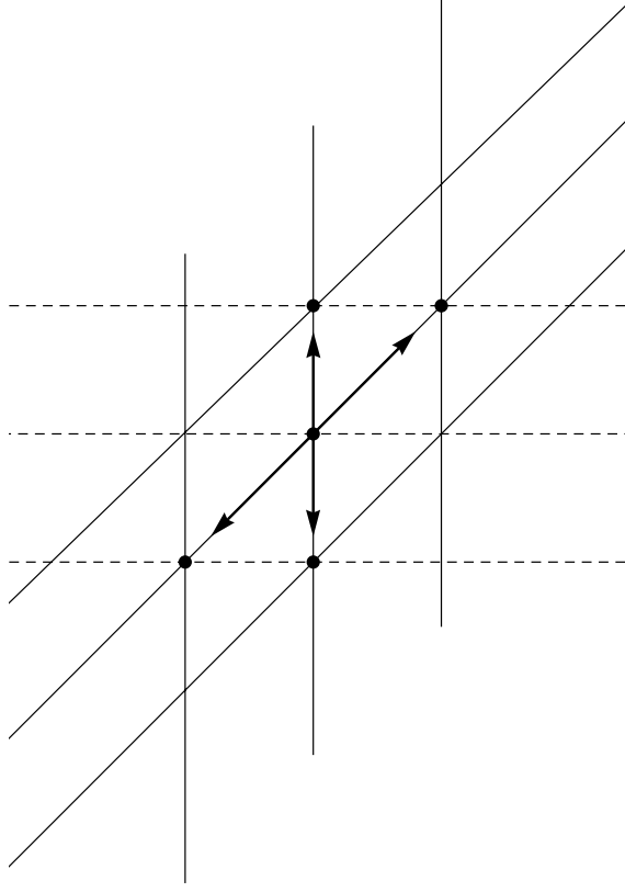
Figure 3: The deformed square lattice walk steps after the modular transformation.
