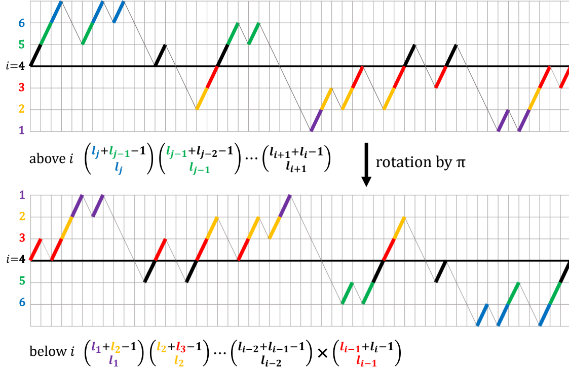
Figure 8: A periodic Dyck path starting and ending at floor i = 4 . The first (blue) up step on floor 6 is connected to the (green) up step on floor 5 at its left, and the next two floor 6 up steps are connected to each other and the floor 5 up step to their left. The steps on floor 5 become “units” with the floor 6 steps attached to them, and are attached to floor 4 (black) up steps to their left. Rotating by \pi , (purple) up steps on floor 1 are connected to (orange) up steps on floor 2 to their left, and similarly for steps on floors 2 and 3 (red). The ordering of up steps on the remaining floors 4 and 3 (except the starting step) is unrestricted.
