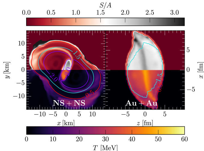
Fig. 2: Distributions of entropy per baryon (top) and temperature (bottom) for a binary neutron-star merger with total mass of 2.8 M_\odot (left) and a Au+Au heavy-ion collision at E_{\text{lab}} = 450 MeV (right). Density contours are shown in units of n_0 . The snapshots refer to t = 3 ms after merger and to t = 5 fm/c after the full collision overlap. Figure modified from Ref. [55].
