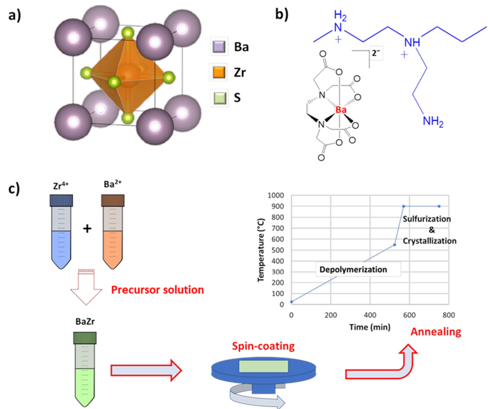
Figure 1. Schematic illustrations of (a) crystal structure of perovskite BaZrS 3 , (b) the polymer (such as PEI) in the solution binds to the metal ions (such as Ba) through electrostatic attraction, hydrogen bonding, and/or covalent bonding, and (c) the major stages of PAD deposition process to synthesize BaZrS 3 films.
