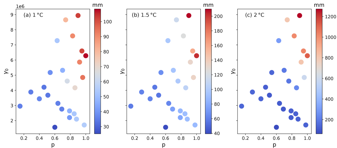
Figure A9. Final (500 years) sea level contribution from the Amundsen under three different synthetic forcing scenarios as a function of \gamma_0 versus p . The panels correspond to the three experiments: 1 °C (a), 1.5 °C (b) and 2 °C (c). Note the different color-bar scales.
