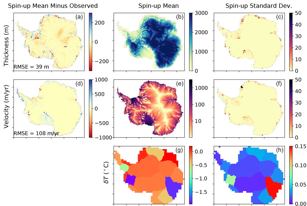
Figure 5. End-of-spin-up statistics: thickness (a, b, c), surface velocity (d, e, f), and \delta T values (g, h). Columns show the end-of-spin-up mean minus observed values (a, d), spin-up mean (b, e, g), and standard deviation (SD) (c, f, h). Spin-up mean and SD are computed across all 25 p and \gamma_0 ensemble members. Observed thickness is from the BedMachine Antarctica V2 (Morlighem et al., 2020), and observed velocities are from Mouginot et al. (2014).
