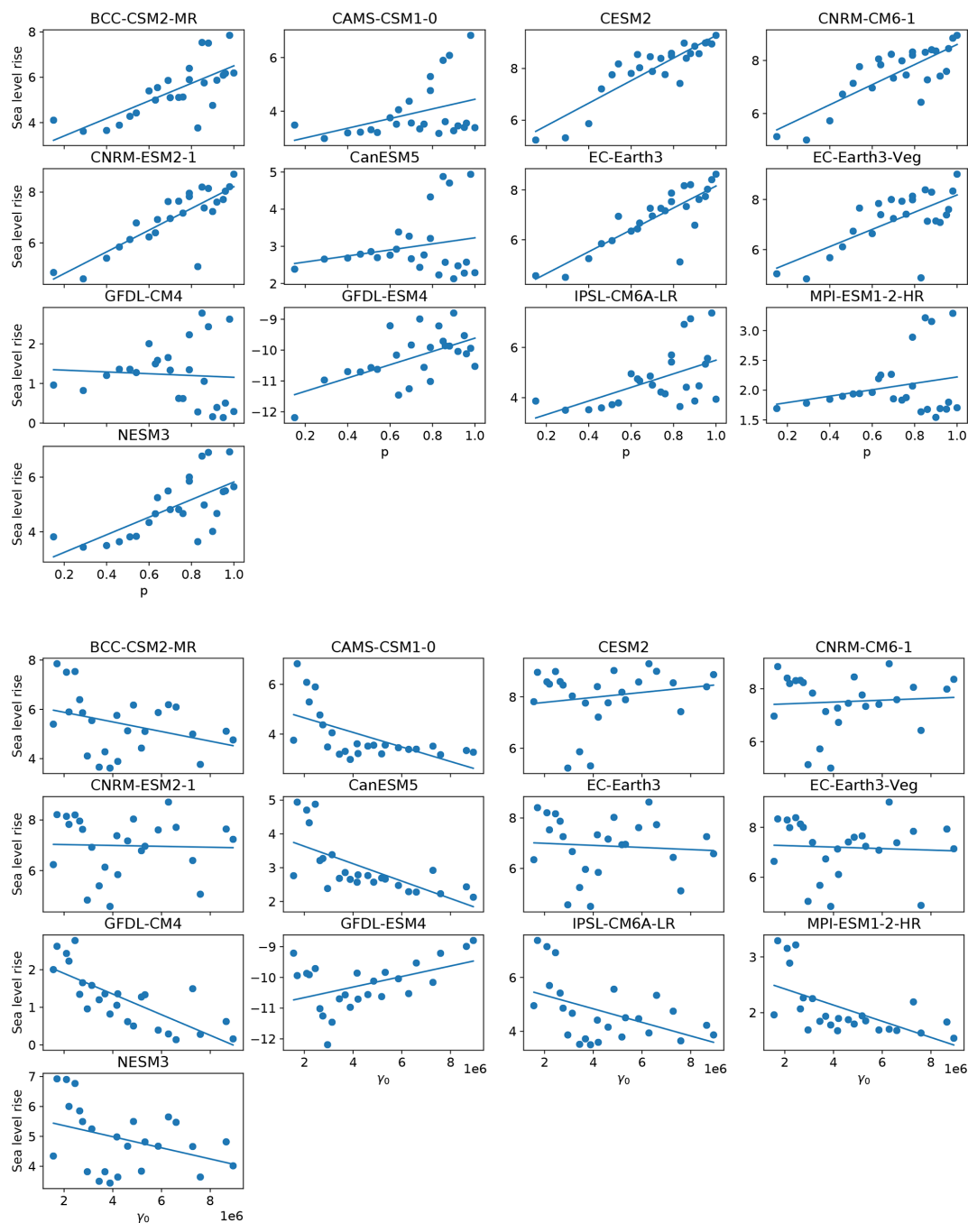
Figure A7. SLR as a function of p and \gamma_0 in the Antarctic Peninsula (AP) region.
