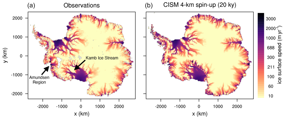
Figure 1. Observed (Rignot et al., 2011) (a) and modeled (b) Antarctic surface speed ( \text{m yr}^{-1} , log scale) for the initial spin-up state used to initialize our 25 ensemble spin-ups (using p = 0 and \gamma_0 = 2062539 ). The root mean square error between observed and modeled velocity is 128.7 \text{ m yr}^{-1} . White patches represent missing data.
