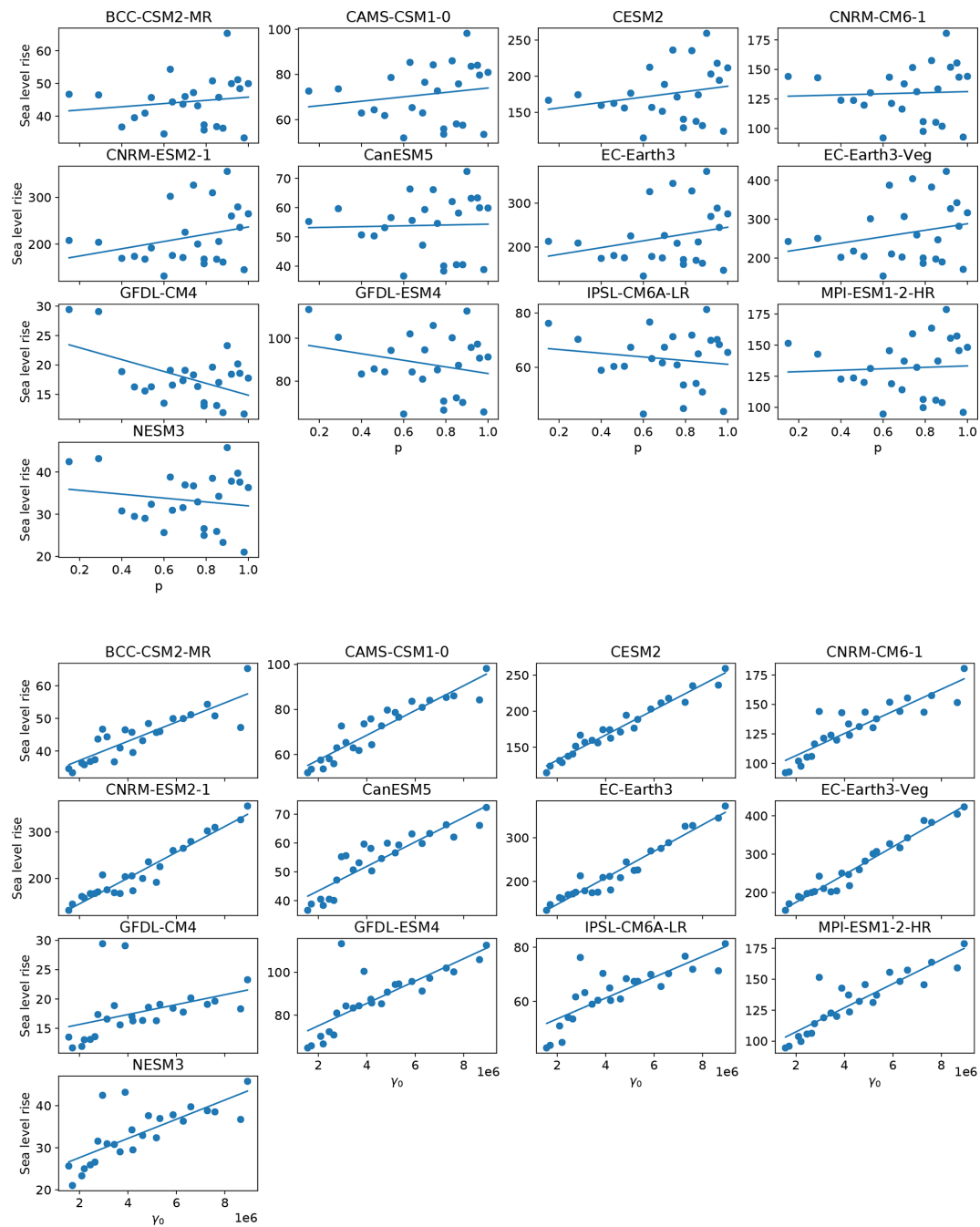
Figure A8. SLR as a function of p and \gamma_0 in the East Antarctic Ice Sheet (EAIS) region.
