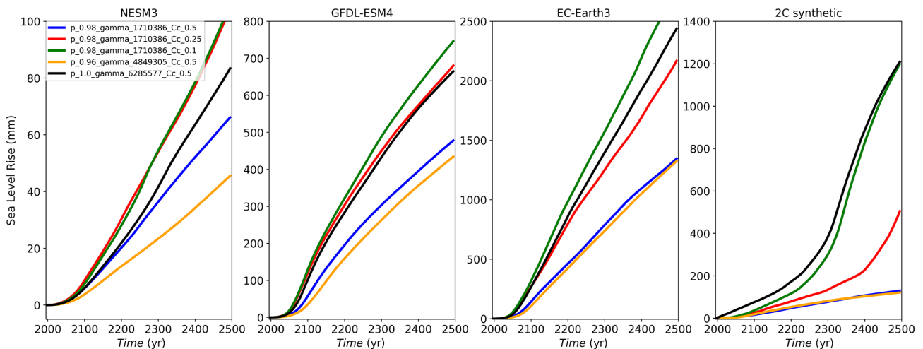
Figure A10. Sea level rise experiment using low (NESM3), moderate (GFDL–ESM4), and high (EC–Earth3) CMIP6 climate scenarios and 2 °C synthetic experiment showing results using high p and low \gamma_0 values, with C_c = 0.5, 0.25, 0.1 (blue, red, green, respectively) and high p , C_c = 0.5 , and mid/high \gamma_0 values (orange and black, respectively). The results show the following: (1) for fixed p and \gamma_0 , lower C_c values lead to a stronger sea level response (the exceptional behavior seen with NESM3 might be due to the low and negative TF forcing in the Amundsen region); (2) for the three CMIP6 forced experiments, lowering C_c by a factor of 5 is not enough to match sea level contribution produced by the spin-ups using higher \gamma_0 values; (3) in the 2 °C synthetic experiment, the results with C_c = 0.1 lead to similar sea level response compared with the experiment with high \gamma_0 .
