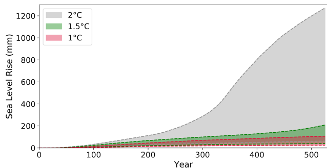
Figure 13. Range of sea level rise for all ensemble members, shaded color indicates the synthetic thermal forcing experiment.
