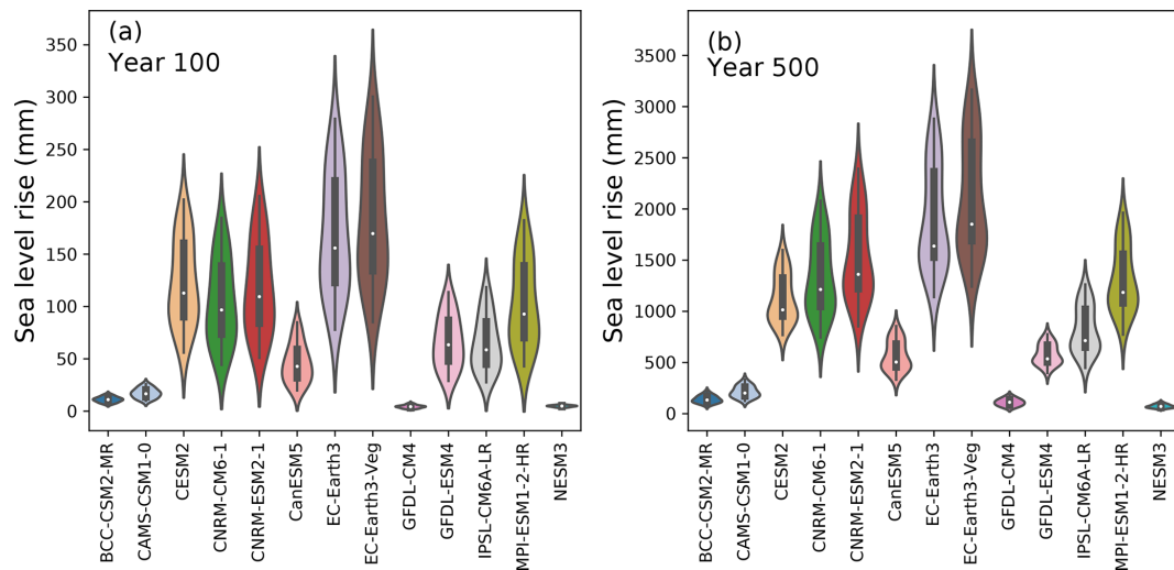
Figure 8. Model spread of SLR after (a) 100 years and (b) 500 years. Note the different y scale in the panels.
