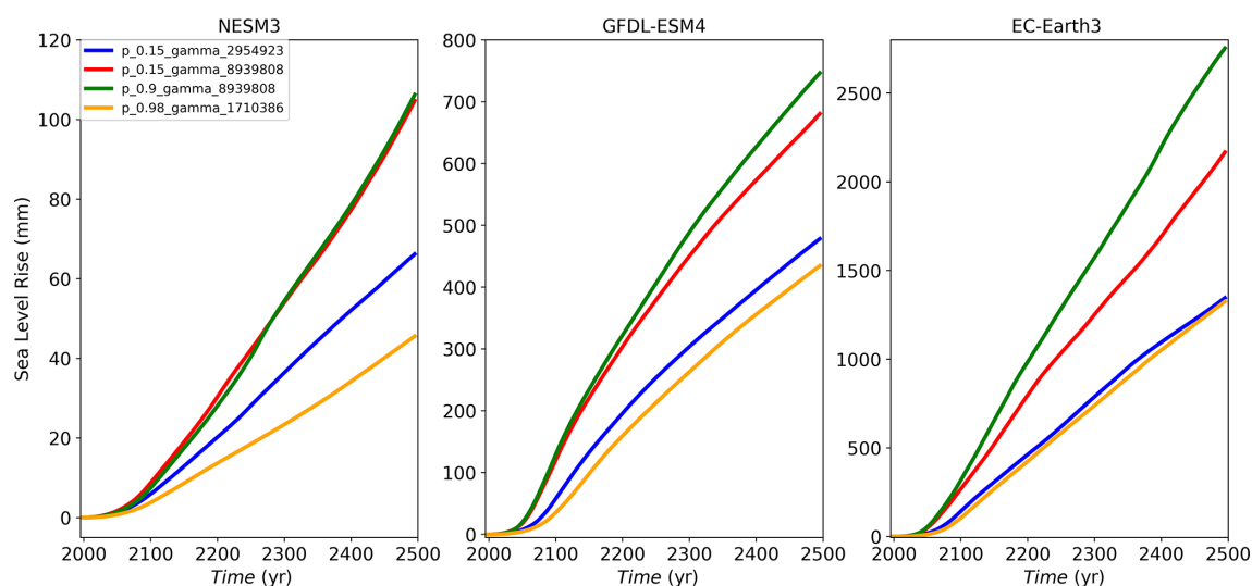
Figure A1. Sea level rise experiment using low (NESM3, a ), moderate (GFDL-ESM4, b ) and high (EC-Earth3, c ) CMIP6 climate scenarios, showing results using p/\gamma_0 values that are low/low (blue), low/high (red), high/high (green), and high/low (orange). The results show the following: (1) with low p and high \gamma_0 the sea level response is similar compared to the high p and high \gamma_0 combination for low and moderate forcing; (2) p does influence the results under high forcing scenarios; (3) the sea level response with low p and high \gamma_0 is always larger compared to the response with high p and low \gamma_0 , highlighting the strong influence of \gamma_0 .
