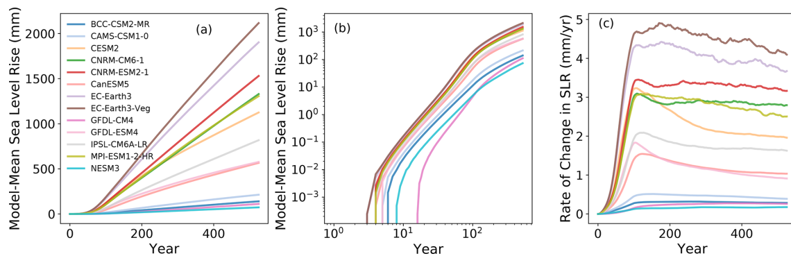
Figure A3. (a) Model-mean sea level rise, (b) model-mean sea level rise on log–log scale and (c) model-mean SLR rate of change ( \text{mm yr}^{-1} ).
