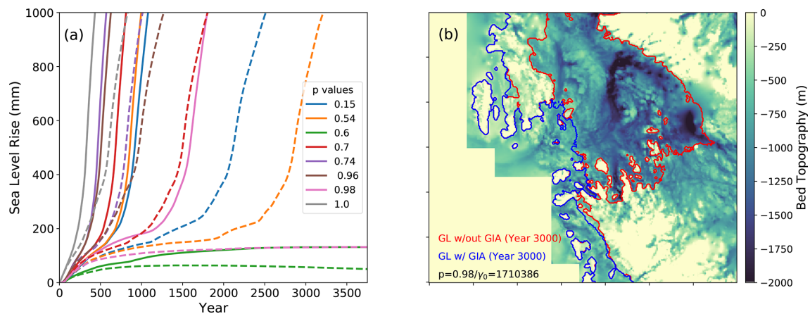
Figure 15. (a) Sea level rise for eight extended simulations with (dashed lines) and without (solid lines) a GIA model. The y axis is truncated at 1 m sea level rise to emphasize GIA-related delays of several centuries. (b) Amundsen region grounding line location evolution over the 2 °C synthetic run for p = 0.98/\gamma_0 = 1710386 without GIA (red) and with GIA (blue) after 3000 years of simulation time. The shaded background shows seafloor topography (m) without isostatic adjustment. Negative values indicate a bed below sea level.
