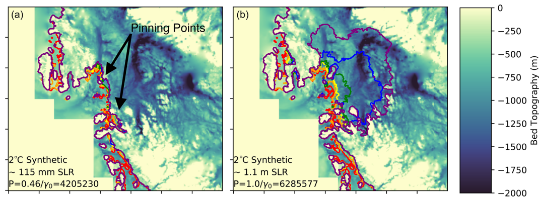
Figure 14. Grounding line location evolution over the 2 °C synthetic run for (a) p = 0.46/\gamma_0 = 4205230 and (b) p = 1.0/\gamma_0 = 6285577 . Red, orange, yellow, green, blue and purple contours indicate years 0 to 525 at roughly 100-year intervals. Shaded background shows seafloor topography (m). Negative values indicate below sea level. Note that the ice in this area is largely grounded below sea level.
