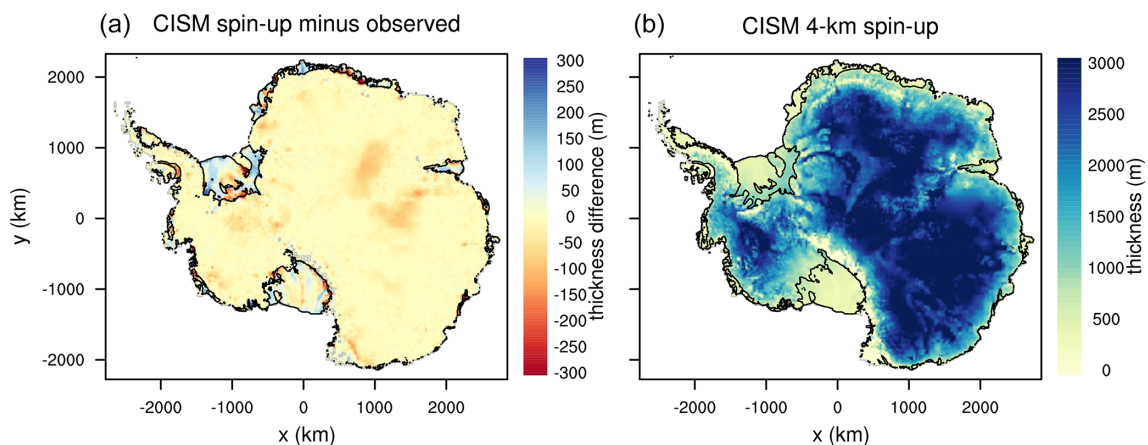
Figure 2. Difference between modeled and observed ice thickness (a) and modeled ice thickness (b) for the initial spin-up state used to initialize our 25 ensemble spin-ups (using p = 0 and \gamma_0 = 2062539 ), with root mean square error 51.8 m. Observations are from the BedMachine Antarctica data set (Morlighem et al., 2020).
