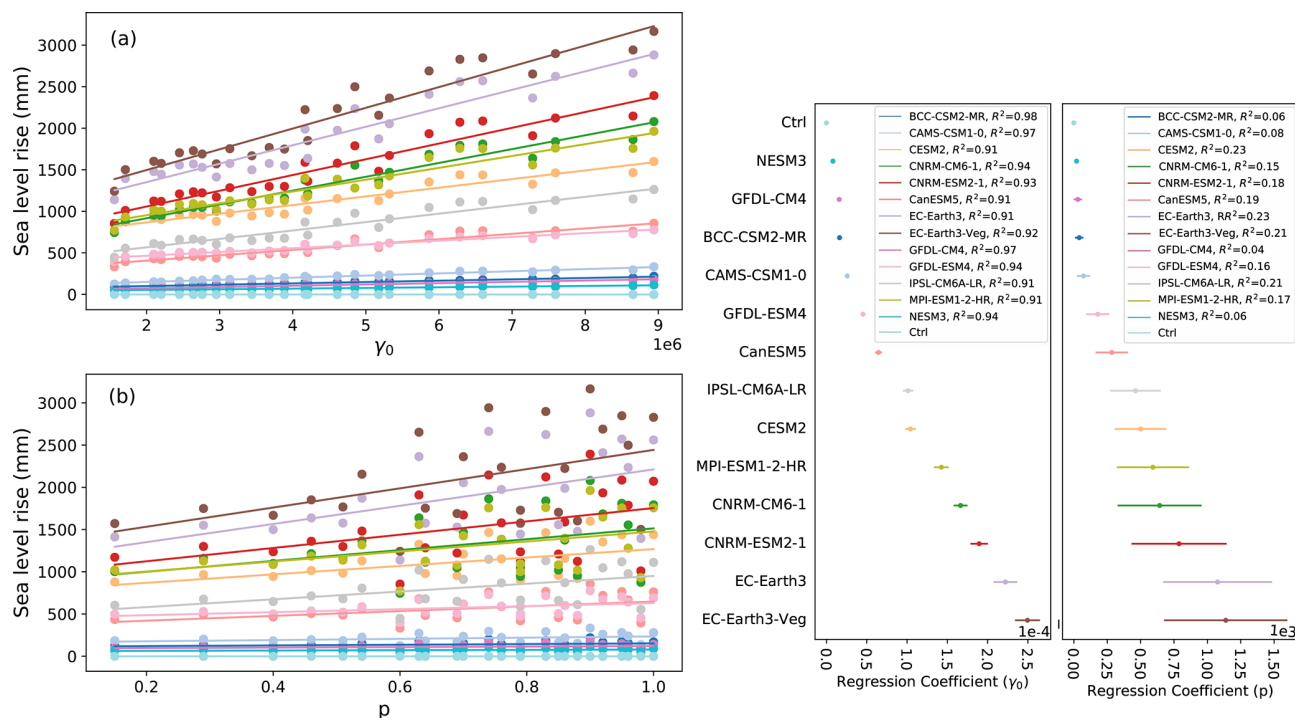
Figure 10. Continental SLR as a function of (a) \gamma_0 and (b) p with best linear fits. Panels on right show the regression coefficients for the model fits along with their error bars. The R^2 value associated with the best fit line is also shown in the legends.
