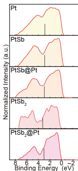
Figure 4. (a) X-ray photoelectron spectroscopy (XPS) valence band spectra. The gray vertical lines designate the valence band center ( \epsilon_d ). The Fermi level is at 0 eV.
