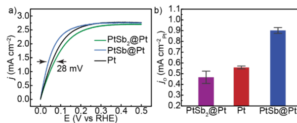
Figure 3. Hydrogen oxidation performance of Pt, PtSb@Pt, and PtSb 2 @Pt measured by (a) linear sweep voltammetry normalized by the geometrical area on a rotating-disk electrode at 1600 rpm and a sweep rate of 5 mV s -1 , and (b) the mass-transport-corrected exchange current density ( j o ) normalized by the electrochemically active surface area on a Pt basis.
