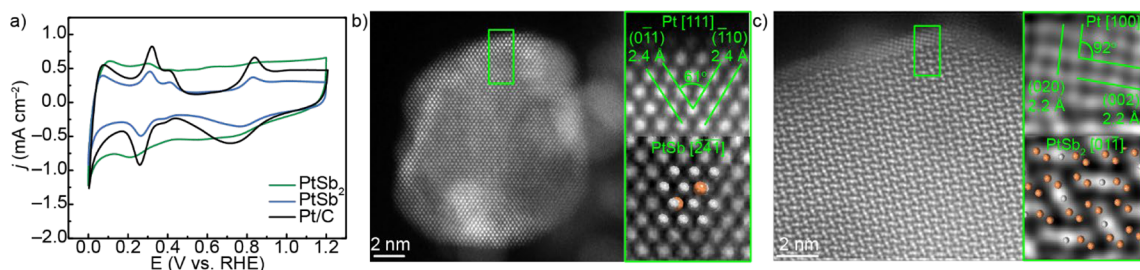
Figure 2. (a) Stabilized cyclic voltammograms (CVs) normalized by the geometric area. (b) STEM/HRTEM image for PtSb nanoparticles after cycling, showing that a PtSb@Pt structure has formed. (c) STEM/HRTEM image for PtSb 2 nanoparticles after cycling, showing that a PtSb 2 @Pt structure has formed.
