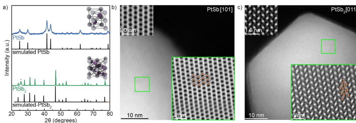
Figure 1. (a) Powder X-ray diffraction (XRD) of PtSb and PtSb 2 nanoparticles supported on carbon. The insets show the unit cells of ordered intermetallic PtSb 2 and PtSb. The simulated XRD patterns of PtSb and PtSb 2 are from ICSD collection codes No. 43105 and No. 16969, respectively. High-resolution HAADF-STEM images of freshly synthesized (b) PtSb and (c) PtSb 2 nanoparticles. The insets on the top left of (b) and (c) are simulated crystal lattices along the PtSb [101] and PtSb 2 [011], respectively. The insets at the bottom right of (b) and (c) with green borders are enlarged regions of the green boxes of the TEM images. An overlay of the simulated crystal are shown in the enlargements of the crystal: the orange spheres depict Sb, and the gray spheres depict Pt.
