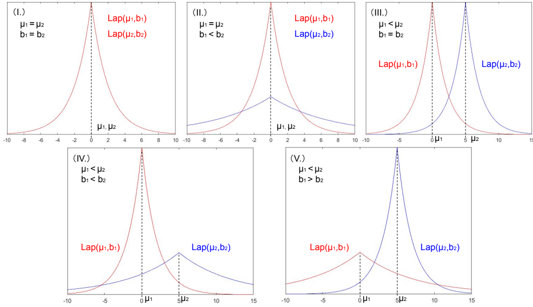
Fig. 9. Five Different Cases of \mu_1 \leq \mu_2 .
