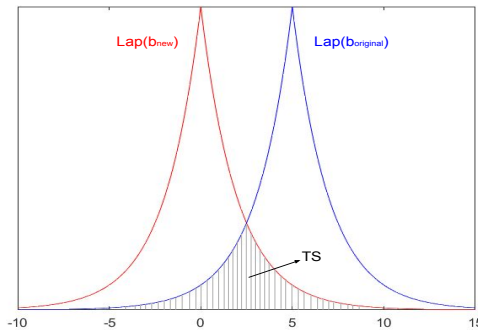
Fig. 4. The GO-BETWEEN Trust Sensitivity.
