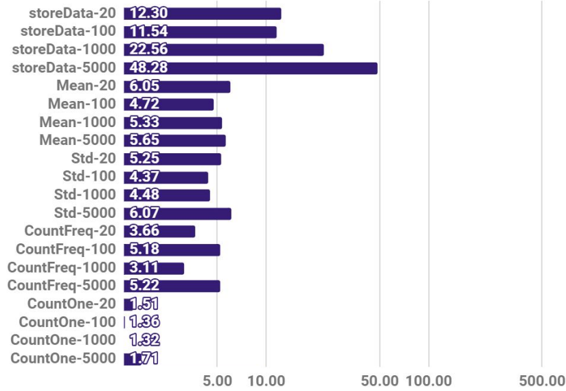
Fig. 7. Performance (log scale with millisecond).
