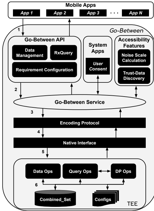
Fig. 5. System Architecture.
