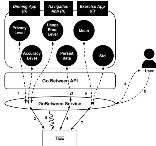
Fig. 6. GO-BETWEEN Programming Model.
