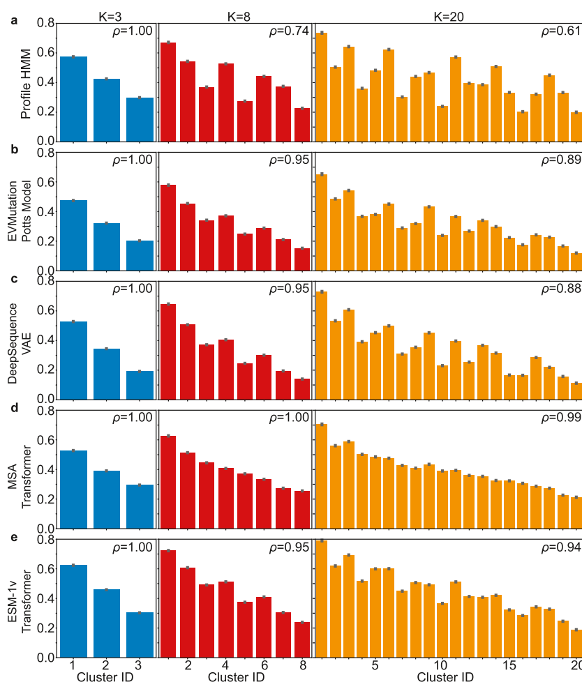
Figure 5. Evolutionary scores capture fitness heterogeneity revealed by K -means for PhoQ data set. K -means is performed using five evolutionary scores as features. Clusters are listed in the descending order of their average fitness, as shown in Figure 3. The y-axis shows the average evolutionary score for (a) Profile HMM, (b) EVmutation, (c) DeepSequence VAE, (d) MSA Transformer, and (e) ESM-1v Transformer. Spearman's correlation between the cluster-wise average fitness and the cluster-wise average evolutionary score is shown in each graph.
