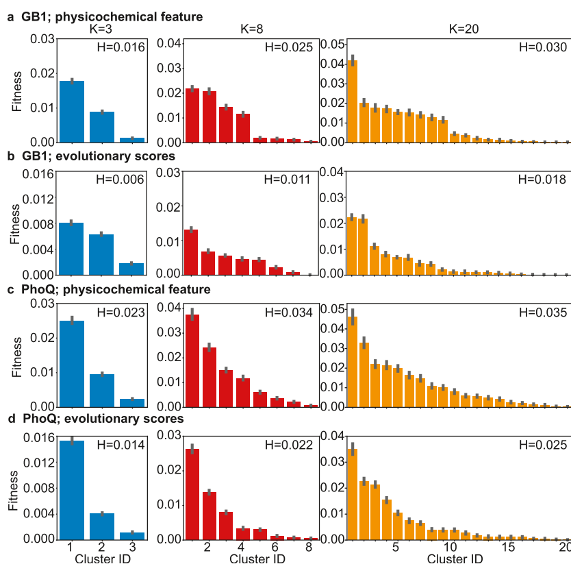
Figure 3. Unsupervised K -means clustering captures fitness heterogeneity. K -means clustering divides the space into K clusters. Plots show average fitness over clusters, where clusters are listed in the descending order of their fitness. Heterogeneity index ( H ) is shown in each subplot. (a) GB1 data set using the physicochemical feature. (b) GB1 data set using five evolutionary scores as features. (c) PhoQ data set using physicochemical features. (d) PhoQ data set using five evolutionary scores as features.
