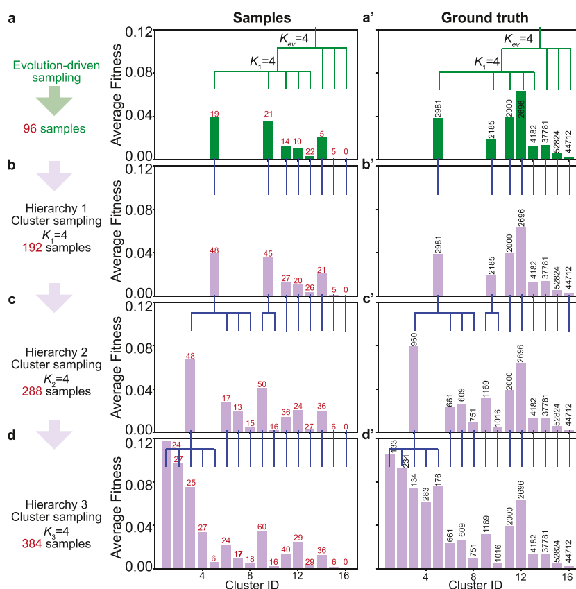
Figure 6. Simulation of procedure of evolution-driven clustering sampling in CLADE 2.0. The simulation is performed with K_{ev} = 4 and K_1 = K_2 = K_3 = 4 . Cluster-wise average fitness for (a–d) selected samples and (a'–d'). Number above each bar shows the number of samples selected in the cluster (red font) or number of samples contained in the cluster (black font).
