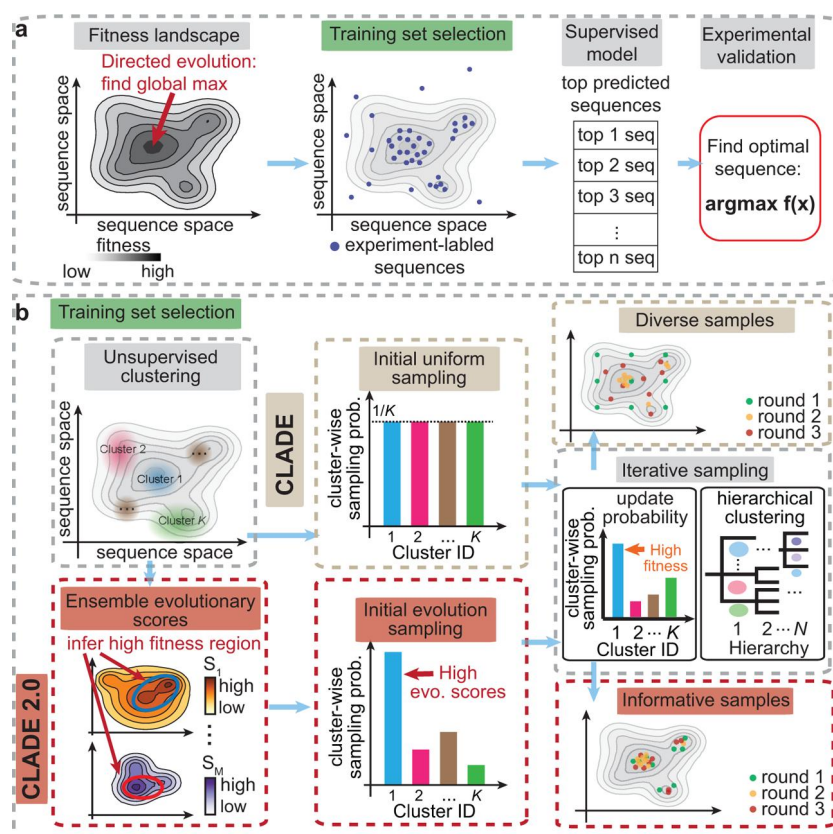
Figure 1. Schematic graph. (a) MLDE searches for a global max sequence in the fitness landscape. It consists of two major steps: training set selection and supervised greedy search to select top sequences. (b) CLADE and CLADE 2.0 are two MLDE strategies that are able to select an informative training set. Initial unsupervised clustering is performed to divide the mutational space into several clusters. CLADE initially uses uniform sampling over clusters. The selected labeled sequences are used to update sampling probabilities and new hierarchical clustering, and the training set is iteratively selected. Evolutionary scores predict fitness landscape in an unsupervised approach and initiate the sampling probability for CLADE 2.0. The later stage clustering sampling of CLADE 2.0 uses the same protocol of CLADE.
