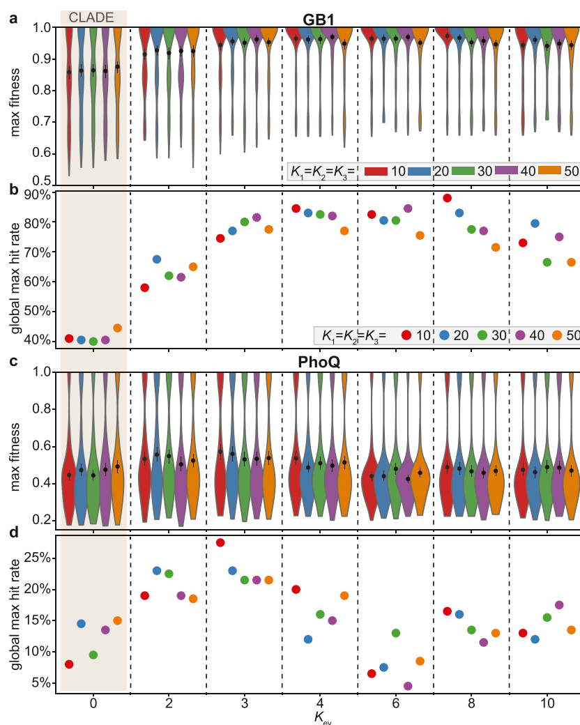
Figure 7. CLADE 2.0 performance on the GB1 data set for (a) expected max fitness and (b) global maximal fitness hit rate; and on the PhoQ data set for (c) expected max fitness and (d) global maximal fitness hit rate. The case with K_{ev} = 0 is equivalent to CLADE. In (a) and (c), violin plots show the kernel density of the max fitness obtained from 200 independent CLADE 2.0 repeats, and the dots show the average with 95% confidence interval shown in the error bars.
