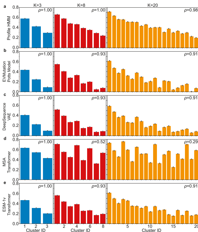
Figure 4. Evolutionary scores capture fitness heterogeneity revealed by K-means for GB1 data set. K-means is performed using five evolutionary scores as features. Clusters are listed in the descending order of their average fitness, as shown in Figure 3. The y-axis shows the average evolutionary score for (a) Profile HMM, (b) EVmutation, (c) DeepSequence VAE, (d) MSA Transformer, and (e) ESM-1v Transformer. Spearman's correlation between the cluster-wise average fitness and the cluster-wise average evolutionary score is shown in each graph.
