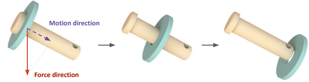
Fig. 2. Our physics-based planning method is motivated by the observation that approximate force directions can be used for disassembly. In this example, the washer can be disassembled from the shaft as long as the force applied has a positive projection along the true disassembly direction, assuming no friction exists.
