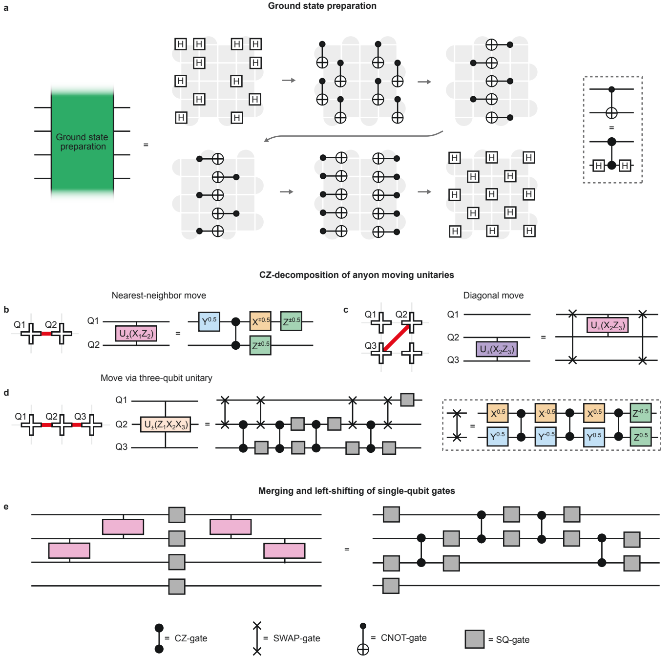
FIG. 6. Ground state preparation and CZ-decompositions. a , Schematic showing the circuit used for preparation of the ground state of the surface code. The protocol is the same as that shown in Ref. 43 , except with the inclusion of Hadamard gates on alternating qubits in the final step, since we use symmetrized stabilizers on the form \tilde{Z}\tilde{X}\tilde{X}\tilde{Z} . b , The unitary needed to move a D3V between two neighboring vertices is realized in the experiment through the use of one CZ-gate and single-qubit rotations. c , When D3Vs are moved diagonally, we include two SWAP-gates, requiring three CZ-gates each. d , Main: The three-qubit unitary used in step VIII in Fig. 3 is equivalent to a combination of single-qubit gates, 4 SWAP-gates and 4 CZ-gates. Right dashed box: decomposition of a SWAP-gate into CZ-gates. e , Adjacent single-qubit gates are merged and shifted left to the nearest CZ-gate.
