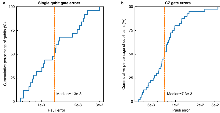
FIG. 2. Gate errors. a,b , Cumulative distributions of the Pauli error for single-qubit ( a ) and two-qubit CZ ( b ) gates. We find median error values of 1.3 \times 10^{-3} and 7.3 \times 10^{-3} for the single-qubit and CZ-gates, respectively.
