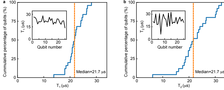
FIG. 1. Qubit relaxation ( T_1 ) and coherence ( T_2 ) times. a,b Cumulative distributions of T_1 ( a ) and T_2 ( b ), where the latter is measured using a Hahn echo sequence. Dashed lines indicate the median values of 21.7 \mu\text{s} for both measures. Insets: T_1 and T_2 plotted against qubit number.
