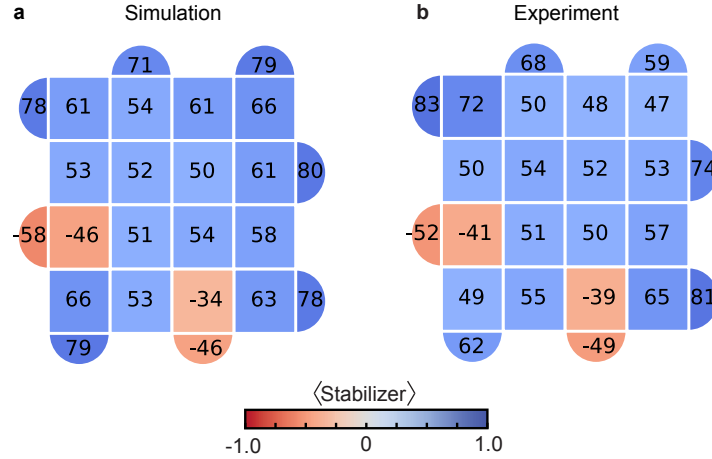
FIG. 7. Simulation of braiding in the presence of noise. a , Simulation results. b , Experimental data (same as in step XII in Fig. 3b in the main text.) We observe relatively good agreement between the simulation and the experimental results, except some discrepancies that are attributed to inhomogeneity of the errors.
