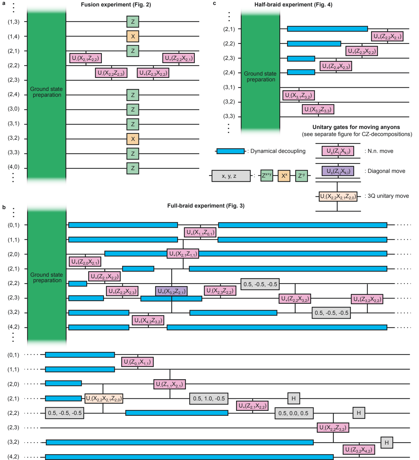
FIG. 5. Circuit details. Circuits used for the fusion experiment (a), the full-braid experiment (b), and the half-braid experiment (c), shown in Figs. 2-4, respectively, in the main text. Turquoise and gray boxes denote dynamical decoupling and phased XZ -gates, respectively. In the full-braid experiment (b), we include five single-qubit rotations to permute \hat{X} , \hat{Y} and \hat{Z} of the three stabilizers touching the moving D3V in steps V-VIII and IX-XI, as well as three Hadamard-gates to return all stabilizers to the original \hat{Z}\hat{X}\hat{X}\hat{Z} -form in XII. See Extended Data Fig. 6 for the circuit used for ground state preparation, as well as details on how the multi-qubit unitary gates used to move anyons are decomposed into CZ-gates.
