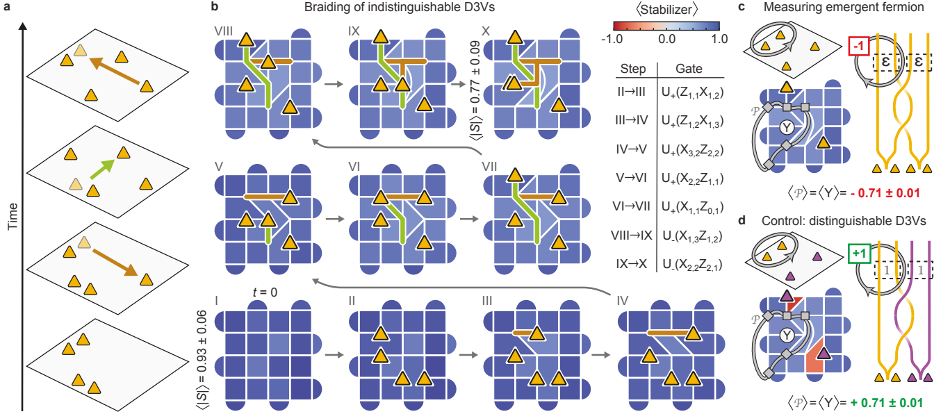
FIG. 9. Alternative protocol for braiding \sigma . a , Schematic displaying the braiding process of the two \sigma -pairs. b , Experimental demonstration of braiding, displaying the values of the stabilizers throughout the process. Two \sigma -pairs, A and B, are created from the vacuum 1 , and one of the D3Vs in pair A is brought to the right side of the grid. Next, a \sigma from pair B is moved to the top, thus crossing the path of the first \sigma , before bringing the \sigma from pair A back again to complete the braid. The diagonal \sigma move performed in step VI is achieved by including two SWAP-gates, corresponding to 6 additional CZ-gates. The yellow triangles represent the locations of the \sigma , while the brown and green lines represent the paths of \sigma from pair A and B, respectively. The average absolute stabilizer value is 0.93 \pm 0.06 and 0.77 \pm 0.09 in the first and last step, respectively. c , After braiding the \sigma , we search for hidden fermions by measuring the Pauli string \hat{\mathcal{P}} (left panels), which here is equivalent to \hat{Y} on the qubit where the two \sigma overlap. The measurement yields \langle \hat{\mathcal{P}} \rangle = \langle \hat{Y} \rangle = -0.71 \pm 0.01 , indicating creation of a fermion. Right: world-lines of braiding process, including non-local measurement based on plaquette violation loop. d , Same as c , but after braiding two distinguishable \sigma , achieved by applying the inverse two-qubit gates when moving the \sigma in pair B. The measurement yields \langle \hat{Y} \rangle = +0.71 \pm 0.01 , indicating no fermion creation.
