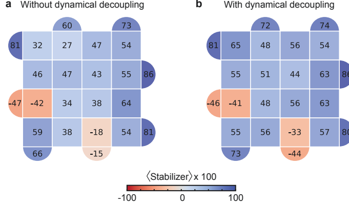
FIG. 4. Dynamical decoupling. a,b , Stabilizer values without ( a ) and with ( b ) dynamical decoupling, after D3V braiding. Dynamical decoupling improves the average absolute stabilizer value from 0.50 to 0.58.
