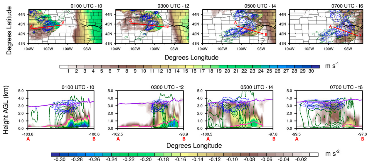
FIG. 12. As in Fig. 8, but for the WSM6 MP scheme.
