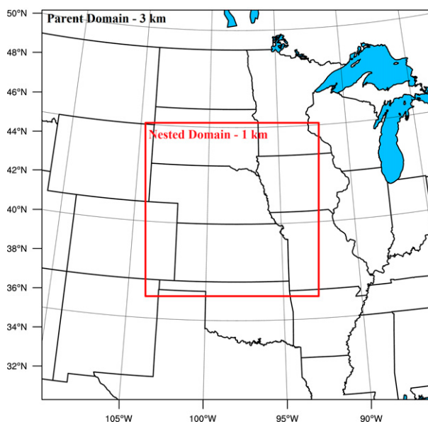
FIG. 1. Example of the WRF-ARW domain configuration for the 9 Jul 2020 case. The parent 3-km domain comprises an area of 2250 \text{ km} \times 2250 \text{ km} , with the inner one-way nested 1-km domain covering 1000 \text{ km} \times 1000 \text{ km} . While the center latitude and longitude placement for the domains varies per case and depends on the location of the observed MCS, the sizes and spatial arrangements of the 3- and 1-km domains are the exact same for all cases.
