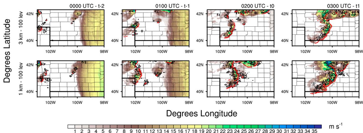
FIG. 15. Progression of the 9 Jul 2020 MCS surface-based cold pool (unfiltered C_{sl} , filled contours; \text{m s}^{-1} ) from the onset of MCS initiation to the early stages of MCS growth ( t - 2 to t_1 , shown from left to right), for the (top) 3 km–100 lev and (bottom) 1 km–100 lev Thompson MP simulations. Black lined contours depict 5+ km AGL (midlevel) updrafts, with red lined contours representing 1–4 km AGL (low-level) updrafts, both exceeding 5 \text{ m s}^{-1} . While the updraft count threshold in MODE was 15 \text{ m s}^{-1} for the 5+ km AGL updrafts, 5 \text{ m s}^{-1} threshold updrafts were shown here for better visibility of the more widespread midlevel updraft coverage.
