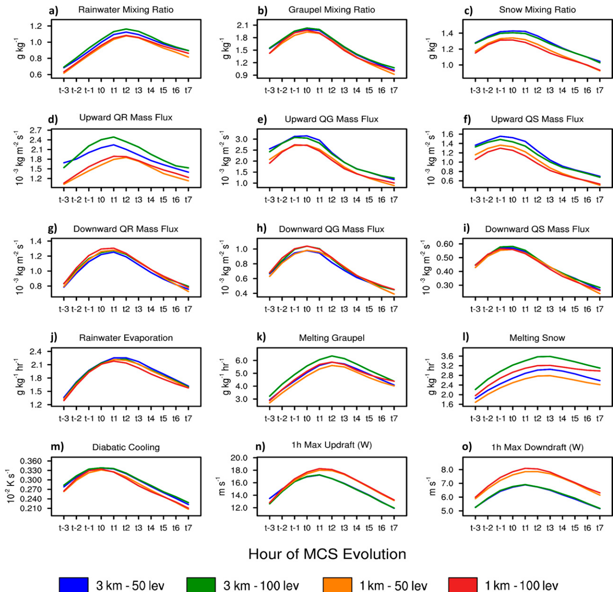
FIG. 11. As in Fig. 7, but for WSM6 MP runs.
