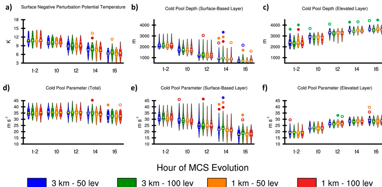
FIG. 10. As in Fig. 6, but for WSM6 MP runs.
