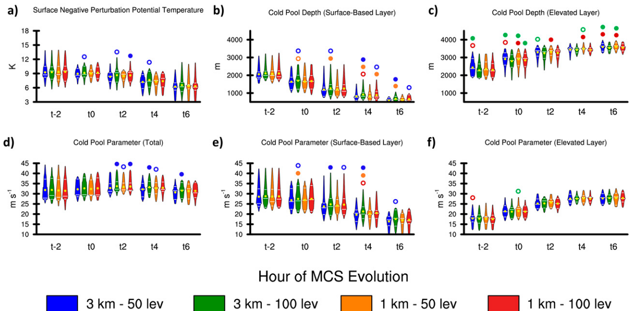
FIG. 6. Violin plots showing the distribution of averaged magnitudes exceeding the 75th percentile among 11 cases for (a) \theta'_{\text{sc}} (K), (b) D_{\text{sl}} (m), (c) D_{\text{elv}} (m), (d) C_{\text{total}} ( \text{m s}^{-1} ), (e) C_{\text{sl}} ( \text{m s}^{-1} ), and (f) C_{\text{elv}} ( \text{m s}^{-1} ). Distributions were calculated for every 2 h of MCS evolution (from 2 h before to 6 h after MCS structure is achieved) for 3 km–50 lev (blue), 3 km–100 lev (green), 1 km–50 lev (orange), and 1 km–100 lev (red). White horizontal lines on the violins delineate the 25th, 50th, and 75th percentiles. Bootstrap statistical significance testing was done between all grid-spacing pairs at each hour, for each variable, where statistical significance is achieved with a p value at or less than 0.05. Filled dots indicate where a sample is statistically significantly larger than the sample represented by the color of the dot. For example, at t4 for D_{\text{sl}} in (b), 3 km–100 lev (green violin) cold pools are significantly deeper than 1 km–50 lev (orange filled dot) and 3 km–50 lev (blue filled dot). Hollow dots represent the same testing philosophy as the filled dots, but for p values between 0.05 and 0.10, and are considered statistically noticeable.
