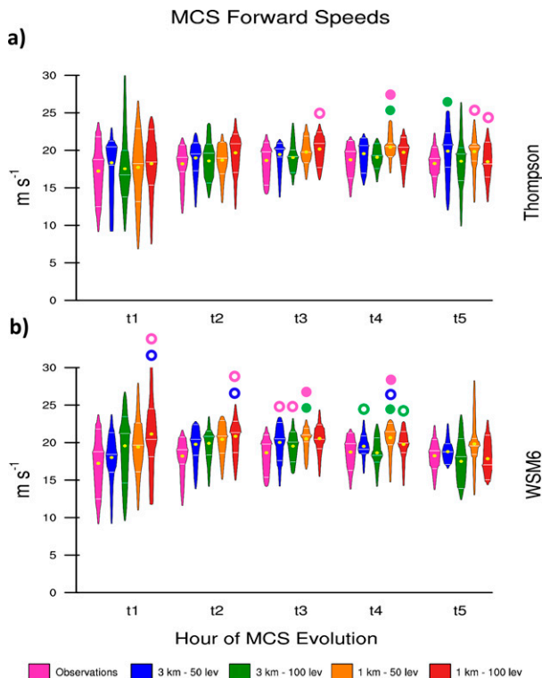
FIG. 6. Violin plots depicting MCS forward speeds ( \text{m s}^{-1} ) for the 11 observed MCSs (pink) and associated simulated MCSs with grid spacings of 3 km–50 lev (blue), 3 km–100 lev (green), 1 km–50 lev (orange), and 1 km–100 lev (red) using (a) the Thompson MP scheme and (b) WSM6 MP scheme, for 1–5 h after MCS initiation (t1–t5). White horizontal lines on the violins delineate the 25th, 50th, and 75th percentiles. The configuration for the violin plots and notation for statistical significance is as in Fig. 4.
