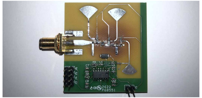
Figure 2. Experimental passive radar system. The signal present on the input is amplified and down-converted in the RF chain. The resulting baseband signal is amplified using an AC-coupled baseband amplifier with fast-start.
