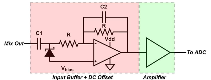
Figure 3. Baseband input buffer and DC offset with included fast-start diode. When power is applied, C1 is charged through the diode. Once the capacitor voltage is within the forward voltage of the diode, the circuit operates normally.
