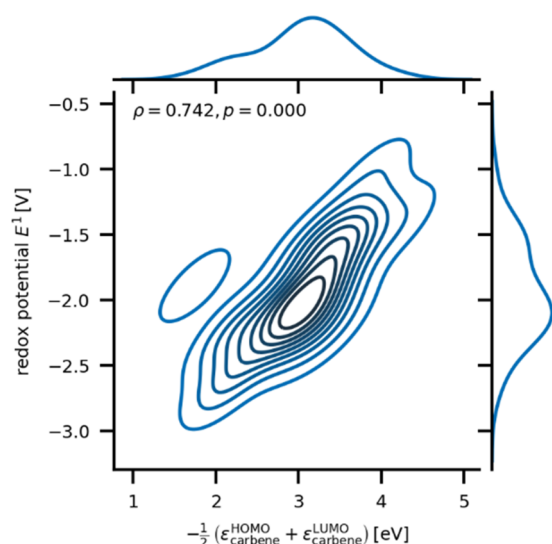
Figure 4. Distribution plot showing the correlation between E^1 and \frac{1}{2}(\epsilon_3^{\text{HOMO}} + \epsilon_3^{\text{LUMO}}) for all computed carbene/ \text{BI}^- pairs, see SI for a full list.
