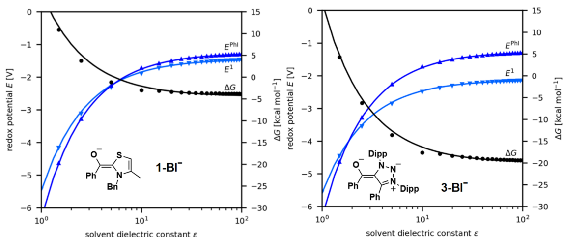
Figure 5. Thermodynamic feasibility of \text{PhI} reduction by \text{BI}^- responds differently with different carbenes which is illustrated for 1 (left) and 3 (right) with the corresponding redox potentials and the redox reaction's \Delta G .
