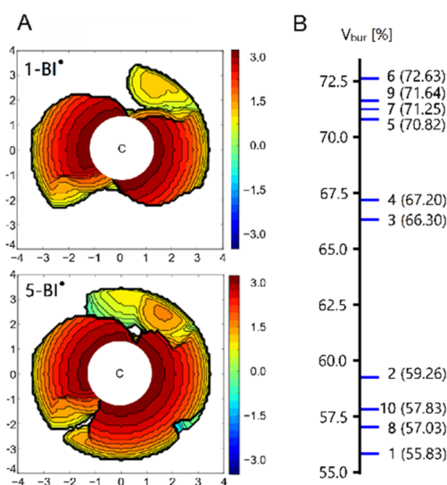
Figure 8. (A) Steric maps of 1-BI* and 5-BI*. (B) Buried volumes of BI* derived from carbenes 1–10.
