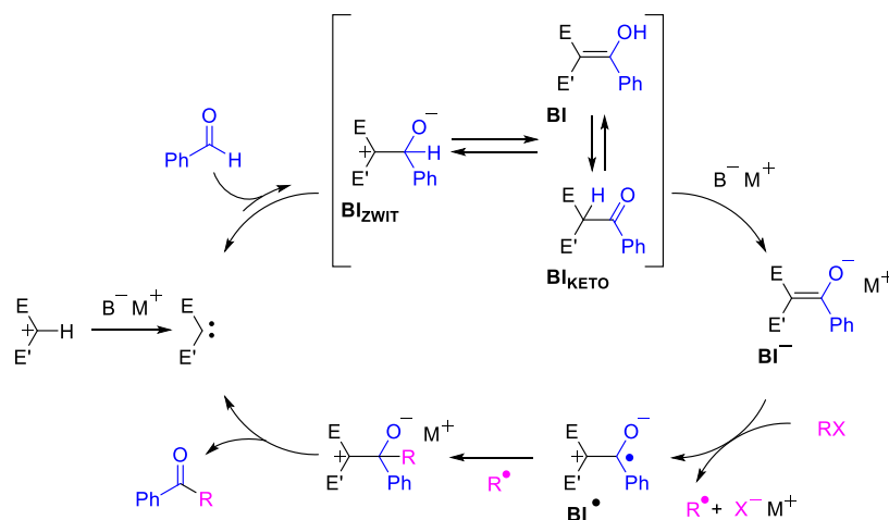
Figure 1. Catalytic cycle for carbene oxidative organocatalytic reactions.
