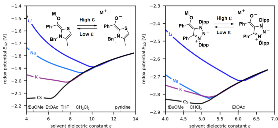
Figure 6. Influence of the cation (Li, Na, K, Cs) on the first reduction potential of \text{BI}^-\text{M}^+ salts derived from carbenes 1 (left) and 3 (right) with the solvent polarity.
