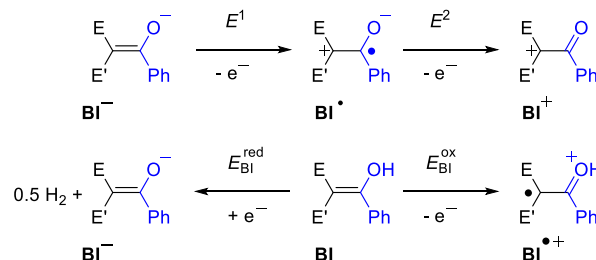
Figure 3. First and second oxidation of BI - (top); reduction and oxidation of BI (bottom).
