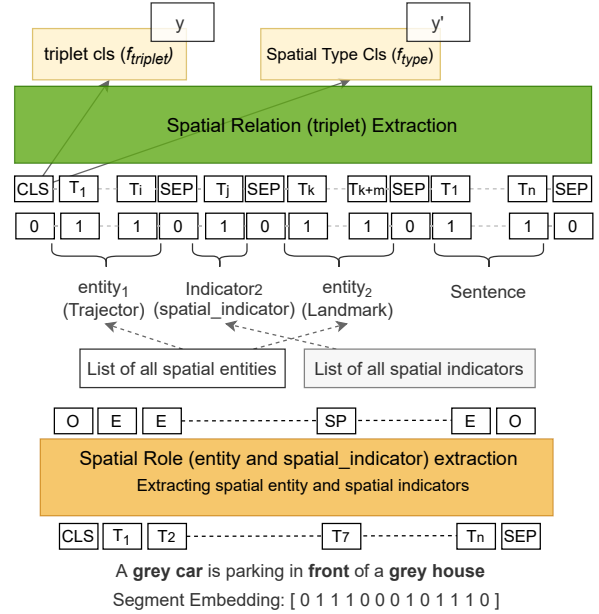
Figure 3: Spatial role labeling model includes two separately trained modules. E: entity, SP: spatial_indicators. As an example, triplet (a grey house, front, A grey car) is correct and the “spatial_type = FRONT”, and (A grey car, front, a grey house) is incorrect, and the “spatial_type = NaN”.
