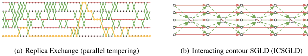
Figure 1: A comparison of communication costs between replica exchange (RE) and ICSGLD. We see RE takes many iterations to swap with all the other chains; by contrast, ICSGLD possesses a pleasingly parallel mechanism where the only cost comes from sharing a light message.
