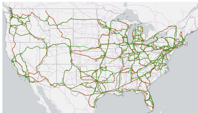
Figure 4: Recreation of the InterTubes long-haul fiber optic cable routes (in brown), the iGDB shortest-path routes that most closely (within 25 miles) follow the InterTubes long-haul links (in green), and the iGDB shortest-path links that do not closely follow the InterTubes links (in purple).
