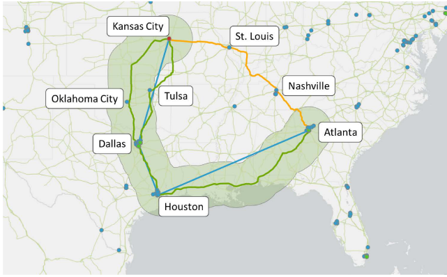
Figure 7: Kansas City to Atlanta traceroute path (blue), inferred physical path through Tulsa, OK or Oklahoma City, OK (green), and shortest practical physical path (orange). AS metro locations depicted as circles with: AS174 (blue), AS12186 (red), AS20473 (green), and AS64199 (purple).
