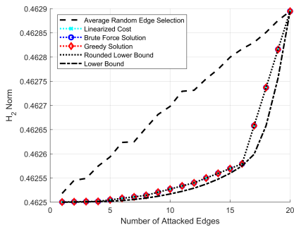
Fig. 4: This figure presents results for bilinear dynamics (2) with topology given by the 10-node ring digraph (Fig. 3). We compare the three proposed methods (linearized cost, greedy algorithm and rounding of lower bound solution) for solving the optimization problem (17) with the actual global minimum obtained through brute force.
