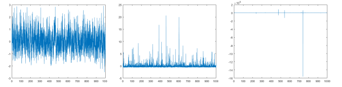
Fig. 2: This figure shows how changing the value of the bilinear term k in the single-input single-output (SISO) bilinear system (16) affects the evolution of state x over time. The system is subjected to Gaussian white noise disturbances \eta and v , with constants a = 1 and b = 1 . The subplots from left to right correspond to k values of 0.1, \sqrt{2} , and 10.
