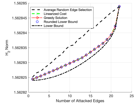
Fig. 6: This figure presents results for bilinear dynamics (2) with topology given by Fig. 5. We compare the three proposed methods (linearized cost, greedy algorithm and rounding of lower bound solution) for solving the optimization problem (17) with the proposed lower bound and the random edge selection. In this case, the bilinear matrices N_k 's are weighted to satisfy Assumption 1 and all methods perform similarly.
