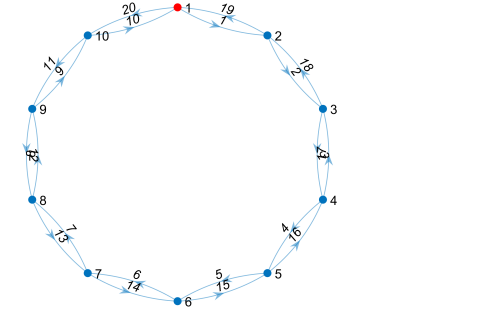
Fig. 3: The directed 10-node ring graph used in Example 1. Node 1, highlighted in red, is the one under the effect of an additive disturbance and all edges are vulnerable.
