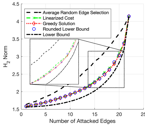
Fig. 7: This figure presents results for bilinear dynamics (2) with topology given by Fig. 5. We compare the three proposed methods (linearized cost, greedy algorithm and rounding of lower bound solution) for solving the optimization problem (17) with the proposed lower bound and the random edge selection. In this simulation, the bilinear matrices N_k 's are unweighted but the dynamics still respect Assumption 2.
