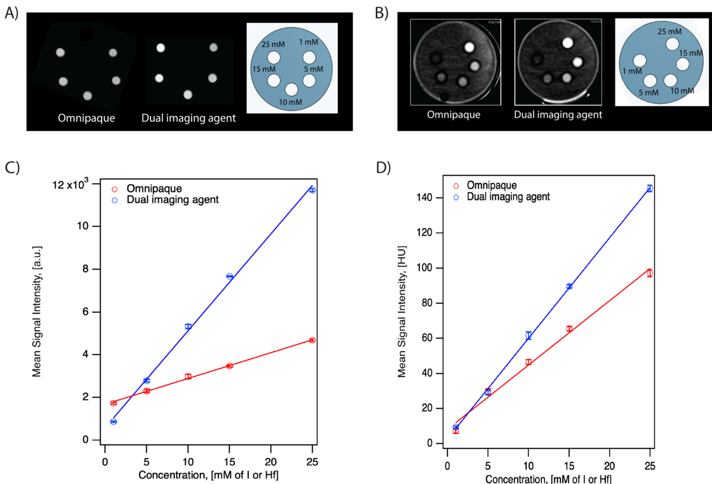
Figure 5. Evaluation of CT performance of the dual imaging agents and Omnipaque at various concentrations in different scanners IVIS® Spectrum In Vivo Imaging System data is shown in A) and C) while Aquilion ONE GENESIS SCT data is shown in B) and D). Representative grayscale images for the dual imaging agents and Omnipaque at various concentrations were presented in A) and B), while quantitative data are presented in C) and D).
