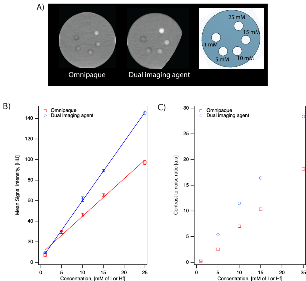
Figure 6. Evaluation of CT performance in Aquilion ONE GENESIS scanner using a dual-energy CT. Representative grayscale CT images (A), CT performance at various concentrations (B), and CNR (C) of the dual imaging agents and Omnipaque.
