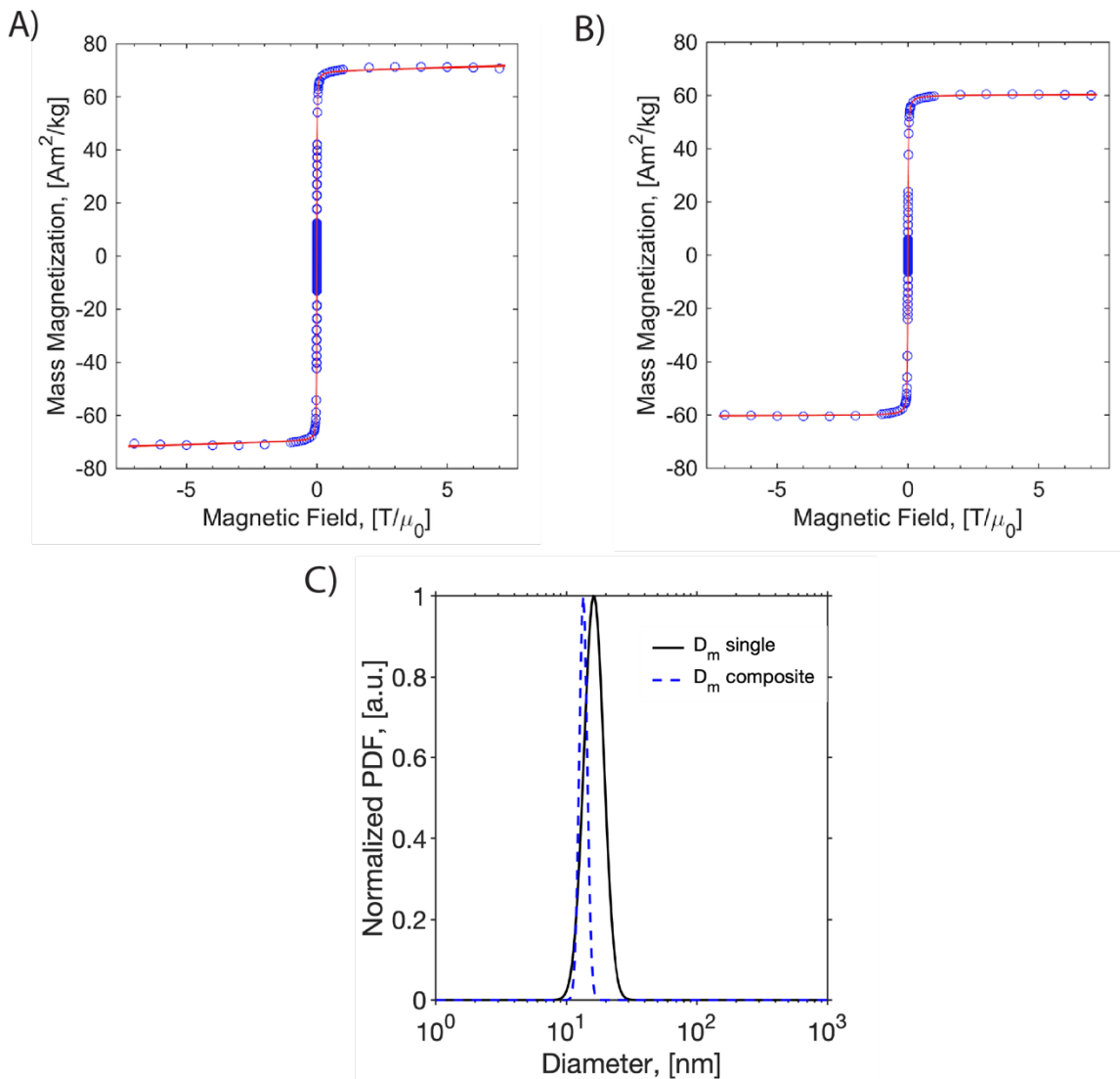
Figure 3. Magnetization versus magnetic field curves obtained using a SQUID magnetometer. A) SPIONs singly coated with PEG-silane. B) dual imaging agents. C) histogram of magnetic diameters for nanoparticles singly coated with PEG (single particles with a polymer corona) and dual imaging agents (composite nanoparticles).
