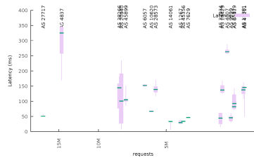
Fig. 20. B-root latency of top talkers by data size (log scale)
