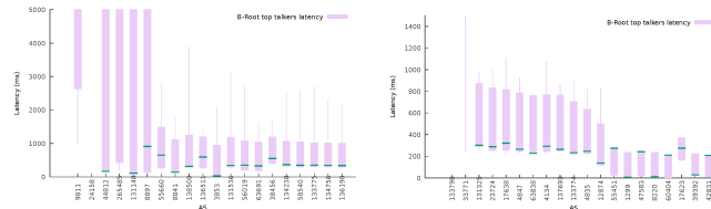
(a) B-root AS latency diversity (b) B-root latency diversity for IPv6 by rank
