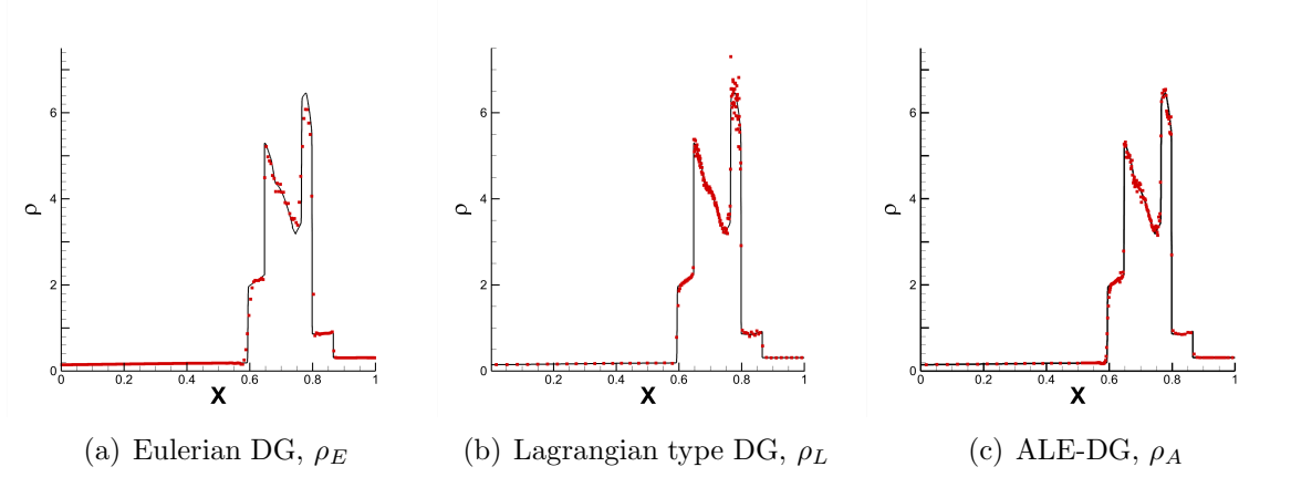
Figure 4.9: Comparison of the reference solution (black solid line) and three third-order DG solutions (red points) for the blast wave problem with N = 200 at time t = 0.038 .
