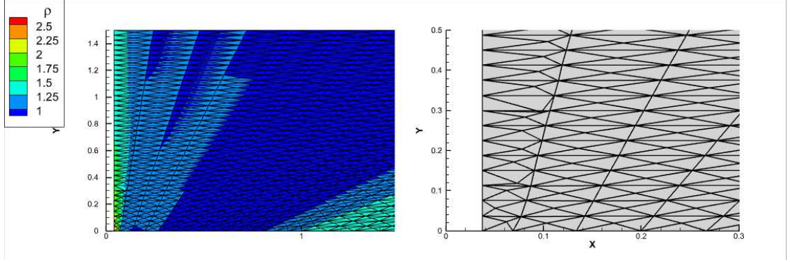
Figure 4.21: The Dukowicz problem of the Lagrangian type DG scheme at t = 0.025 . Right: the zoomed mesh near the left moving boundary.
