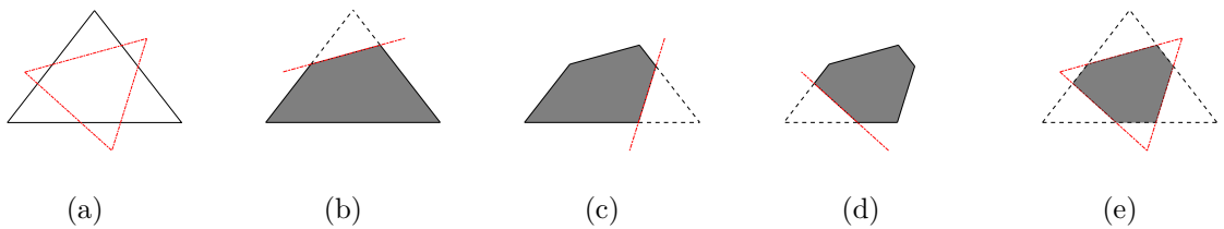
Figure 2.1: The clipping procedure. The black triangle is the target cell, the red triangle is the window cell, the gray shaded polygon is the clipping result.
