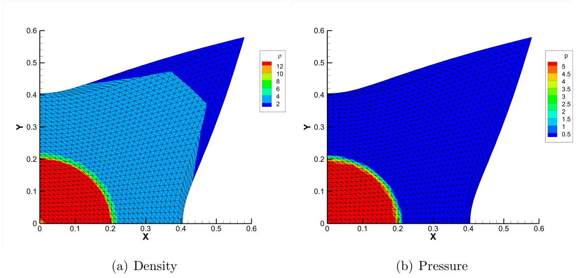
Figure 4.15: The Noh problem of the ALE-DG scheme at t = 0.6 .
