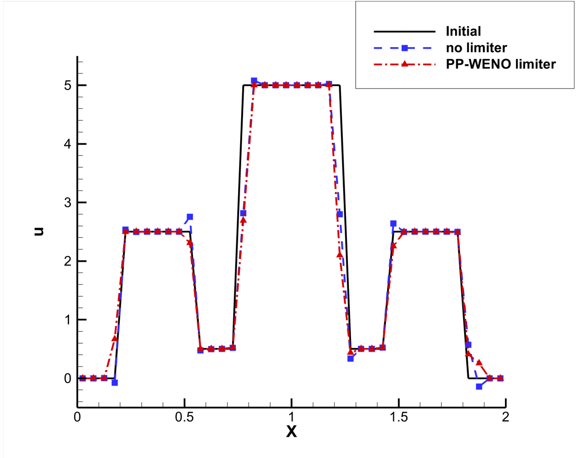
Figure 3.7: The function values at the cut line x = y = z . The black solid line: the initial function; the blue dash line: the remapping results without any limiter \tilde{u}_h^{10}(x, y, z) ; the red dash dot line: the remapping results with the two limiters \tilde{u}_h^{W,P,10}(x, y, z) .
