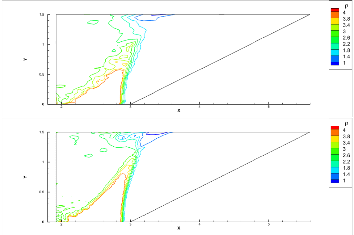
Figure 4.22: The Dukowicz problem of the ALE-DG scheme at t = 1.3 . Upper: 4,800 triangular cells; bottom: 19,200 triangular cells.
