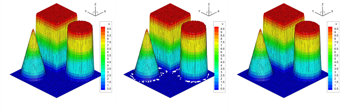
Figure 3.3: Two-dimensional discontinuity test: third-order polynomial projection remapping method with 14,120 triangular cells. Left: the initial function; middle: remapping results without any limiter \tilde{u}_h^{10}(x, y) ; right: remapping results with two limiters \tilde{u}_h^{W,P,10}(x, y) . White symbols represent the cells where the cell-averages are negative.
