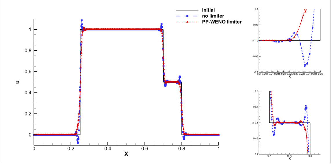
Figure 3.1: One-dimensional discontinuity test: third-order polynomial projection remapping method with 80 cells. The black solid lines are the initial function (3.2), the blue dash lines are the numerical results \tilde{u}_h^{10}(x) without any limiter, the red dash dot lines are the numerical results with the two limiters \tilde{u}_h^{W,P,10}(x) . Top right: the zoomed-in subfigure at x \in [0.2, 0.25] ; bottom right: the zoomed-in subfigure at x \in [0.675, 0.825] .
