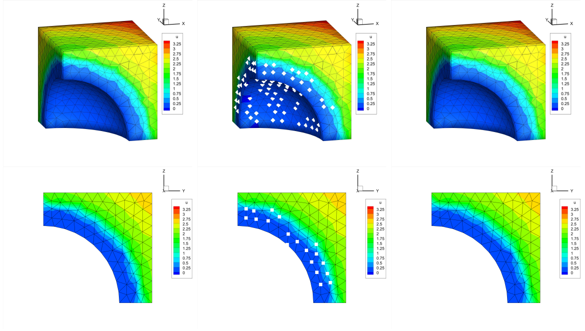
Figure 3.5: Three-dimensional positivity-preserving test: third-order polynomial projection remapping method with 3,938 tetrahedral cells. Left: the initial function; middle: remapping results without any limiter \tilde{u}_h^{10}(x, y, z) ; right: remapping results with the two limiters \tilde{u}_h^{W,P,10}(x, y, z) . The bottom three subfigures are the 2D cut planes at x = 0 and white symbols represent the cells where the cell-averages are negative.
