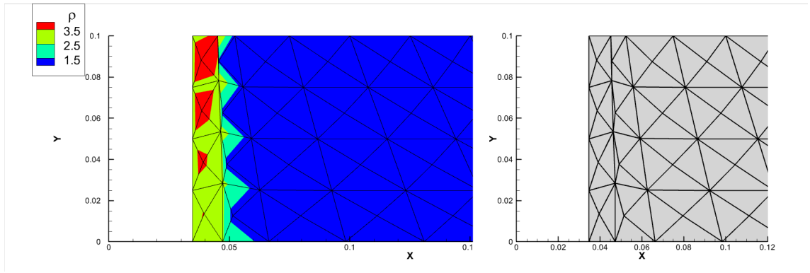
Figure 4.18: The Saltzman problem of the Lagrangian type DG scheme at t = 0.034 . Right: the zoomed mesh near the left moving boundary.
