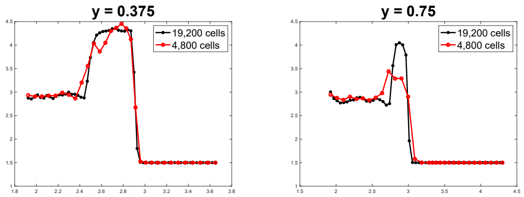
Figure 4.23: The cut line of the Dukowicz problem at y = 0.375 and y = 0.75 .
