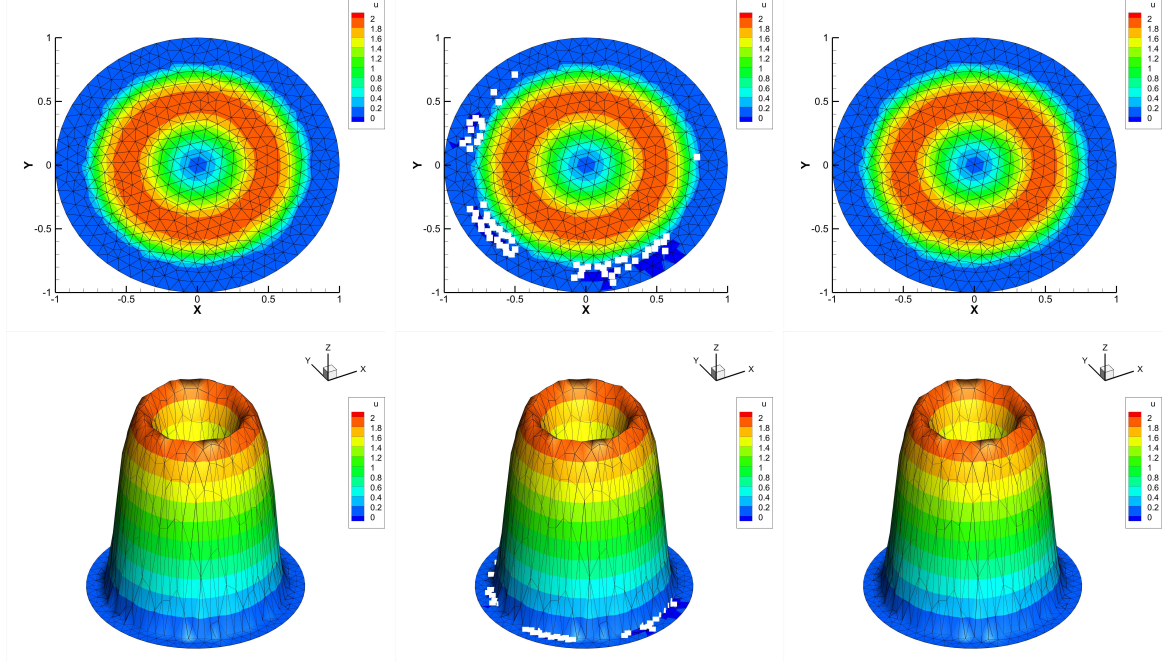
Figure 3.2: Two-dimensional positivity-preserving test: third-order polynomial projection remapping method with 1,016 triangular cells. Left: the initial function; middle: remapping results without any limiter \tilde{u}_h^{10}(x, y) ; right: remapping results with the two limiters \tilde{u}_h^{W,P,10}(x, y) . White symbols represent the cells where the cell-averages are negative.
