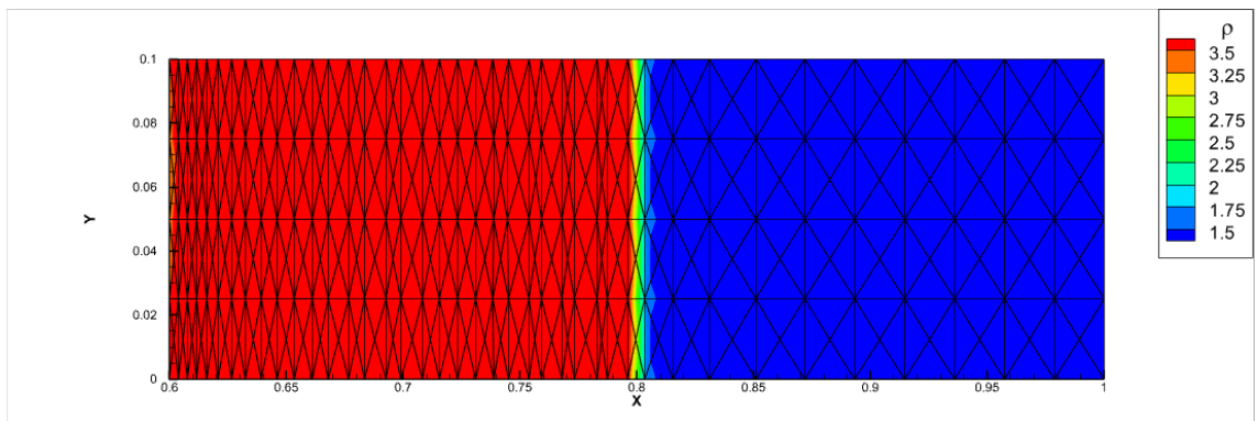
Figure 4.19: The Saltzman problem of the ALE-DG scheme at t = 0.6 .
