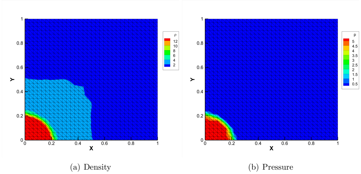
Figure 4.13: The Noh problem of the Eulerian DG scheme at t = 0.6 .
