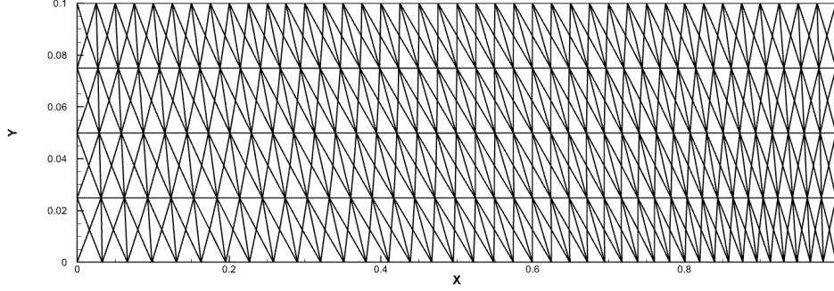
Figure 4.17: The initial Saltzman mesh.
