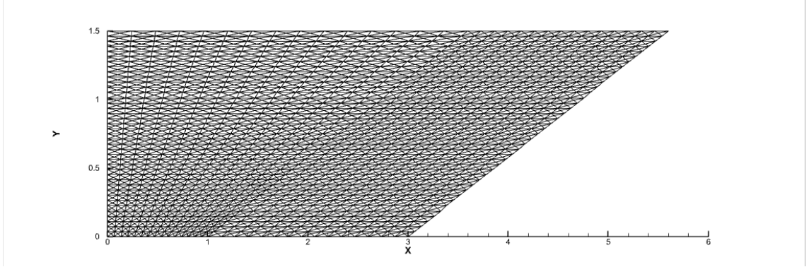
Figure 4.20: The initial Dukowicz mesh with 4,800 triangular cells.
