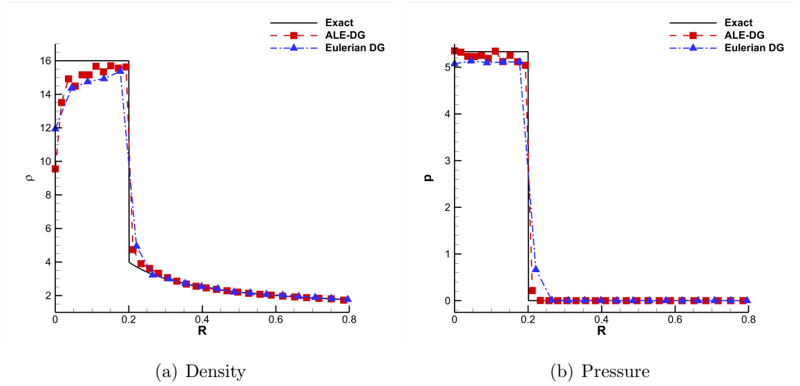
Figure 4.16: The Noh problem at the cut line x = y .
