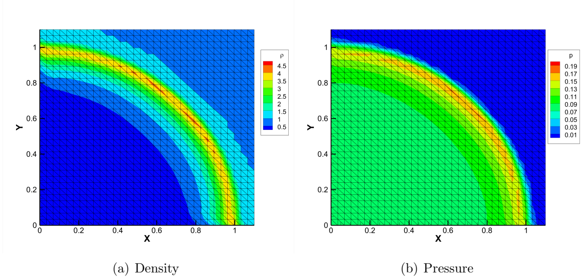
Figure 4.10: The Sedov problem of the Eulerian DG scheme.
