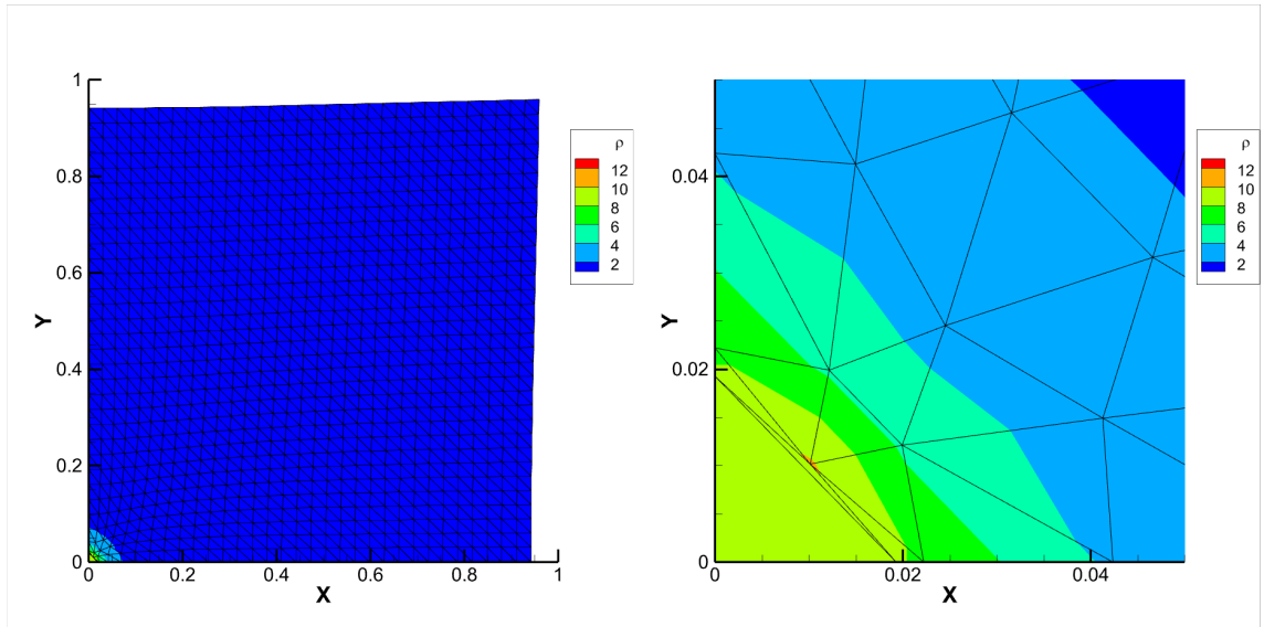
Figure 4.14: The Noh problem of the Lagrangian type DG scheme at t = 0.058 . Right: the zoomed mesh near the origin.
