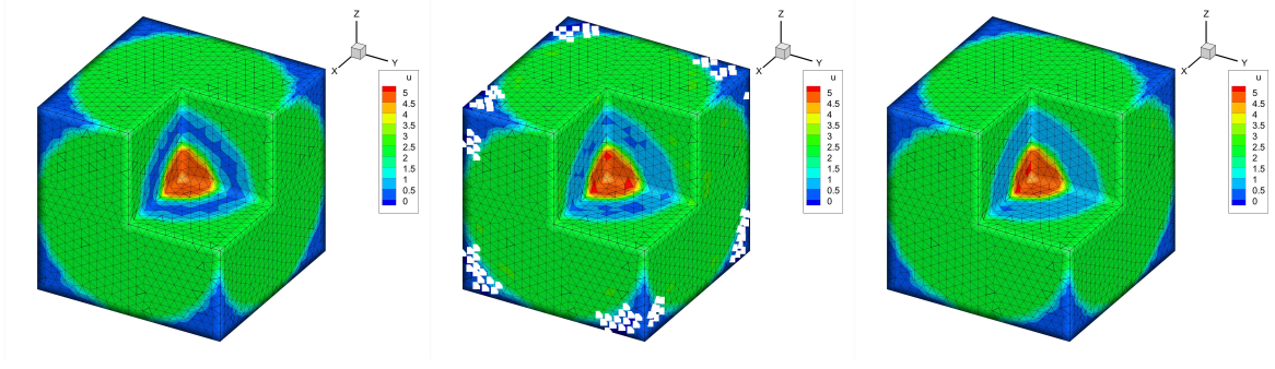
Figure 3.6: Three-dimensional discontinuity test: third-order polynomial projection remapping method with 37,160 tetrahedral cells. Left: the initial function; middle: remapping results without any limiter \tilde{u}_h^{10}(x, y, z) ; right: remapping results with the two limiters \tilde{u}_h^{W,P,10}(x, y, z) . White symbols represent the cells where the cell-averages are negative.
