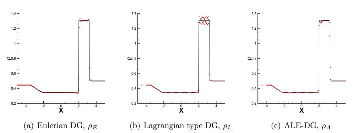
Figure 4.8: Comparison of the exact solution (black solid line) and three third-order DG solutions (red points) for the Lax problem with N = 100 at time t = 1.3 .
