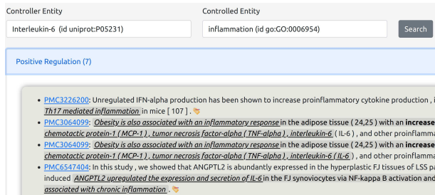
Figure 10: Participant search interface. At the top are the participant search boxes. At the bottom is an “accordion” widget displaying the interactions between both participants, grouped by interaction type.
