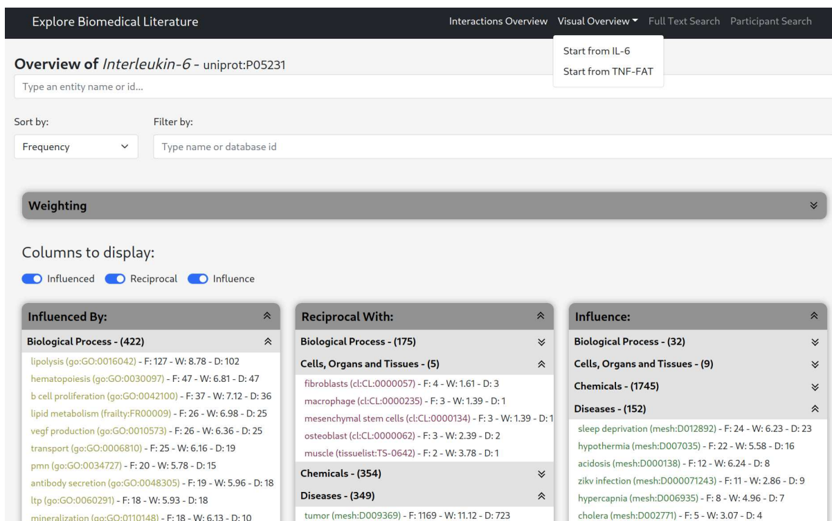
Figure 2: Entity overview interface. The display anchored entity is IL-6. The anchor entity can be changed to search by name or database identifier in the entity search box. The elements in the entity columns can be sorted by multiple criteria and filtered by name or database identifier. The entity columns can be hidden by toggling their display indicator.
