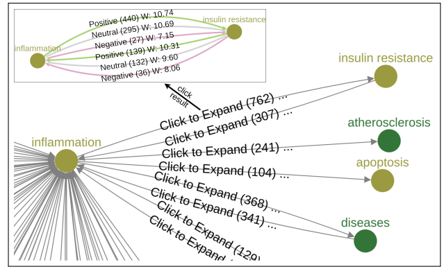
Figure 5: The main figure shows the Node-Link view after double-clicking on Inflammation which fetches additional neighbors. The sub-figure (top-left) shows the Node-Link view of Inflammation and insulin resistance. Polarity is represented by both color and label. Interaction direction is represented by arrows. The numbers correspond to interaction frequency in the database and the value of W is the customized interaction weight (see Fig. 4).
