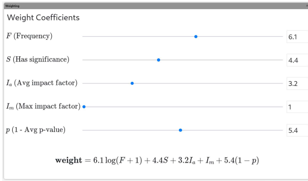
Figure 4: Custom interactions weight widget. Coefficients for each variable can be tuned either by adjusting the slider controls or by directly typing values in. The value returned by this formula is used for all interactions displayed in the current view and for ranking the results. An explanation of each variable is found in §4.1.
