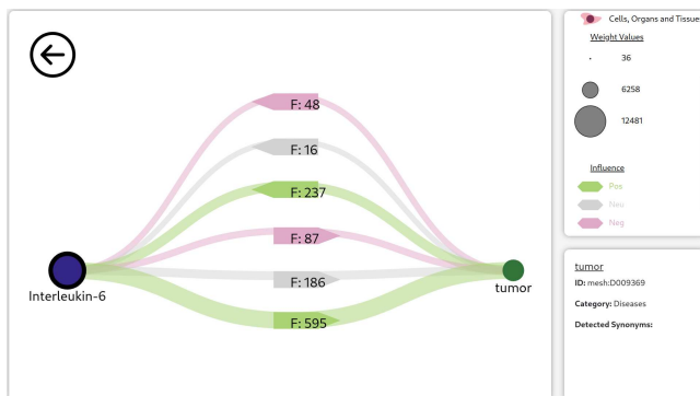
Figure 8: Transition to detailed relation view page. After clicking on 2 nodes (IL-6 and tumor) or an edge between them in the center panel of Fig. 7, all nodes move away from center and the 2 selected nodes create a new visualization from their relations. The arrows indicate the direction of influence, and color denotes type of influence (positive by green, negative by red and neutral by grey). Clicking on these relation edges will show that number of evidences at the bottom panel. The back button on top left corner will transition to Fig. 7.
