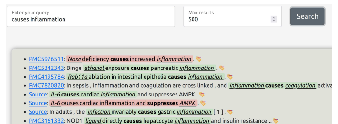
Figure 9: Segment of the full-text search interface. At the top, the search box takes a query and a limit on the number of results. At the bottom, an evidence panel displays the results of the search. Clicking on the text of an interaction will open a page with a Node-Link view of the interaction.
