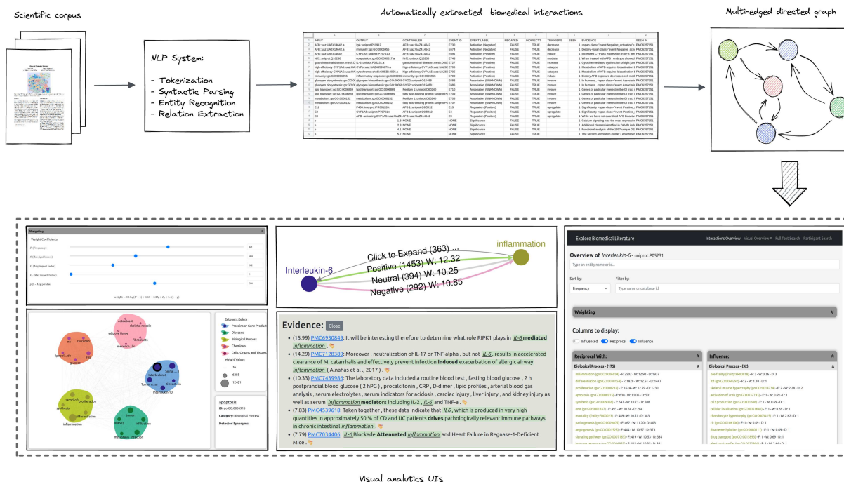
Figure 1: An overview of the proposed system designed to help biomedical researchers to search, visualize and interact with biological networks derived via information extraction tools. The input is texts from scientific papers. An information extraction system is used to detect and assemble structured relations between biological concepts (e.g., chemicals, proteins, diseases). The structured data is then used to create a network, connecting all the individual pieces together. Finally, the domain expert interacts with the network and text via multiple user interfaces, to find relevant interactions and backing evidences.
