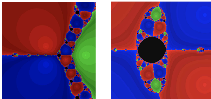
FIGURE 1. For every degree d \geq 3 and every period m \geq 2 there is a polynomial p of degree d so that N_p has a periodic point of period m that attracts a neighborhood of each of its points. Left: The Newton dynamics plane for p(Z) = Z^3 - 2Z + 2 , where N_p(z) = z - \frac{z^3 - 2z + 2}{3z^2 - 2} = \frac{2z^3 - 2}{3z^2 - 2} has an attracting 2-cycle 0 \mapsto 1 \mapsto 0 ; its basin is shown in black. Right: Detail near center.
