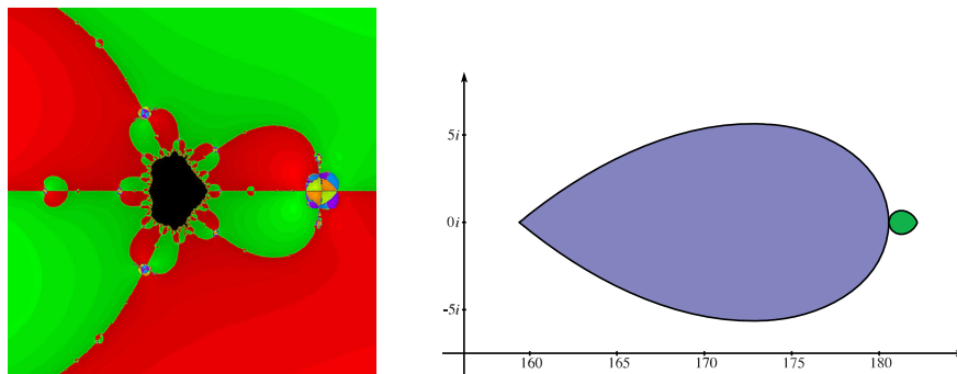
FIGURE 2. Left: The dynamics on the slice of \mathbb{C}^2 given by z_2 = -5.36 , with \operatorname{Re} z_1 \in [-5, -4] and \operatorname{Im} z_1 \in [-0.5, 0.5] . The black region is the intersection with the immediate basin of attraction around a periodic point of order 4 for W_{Z^3+Z+t} with t = 175 . The six colors correspond to the six fixed points given by the various orderings of the three roots; points converging to a fixed point are given the appropriate color and are the brighter the faster they approach the fixed point. Similar colors correspond to fixed points with the same first component.
