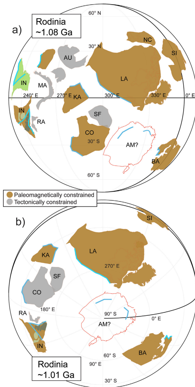
Fig. 13. Rodinia reconstructions at ~1.08 Ga (a) and ~1.01 Ga (b) based on the rotation of paleomagnetic poles in Table 9 to Earth's spin axis using the closest approach method of Meert and Torsvik (2003). For a detailed explanation of Rotation Parameters, see Supplementary Data (S10–S11). AM: Amazonia, AU: Australia, BA: Baltica, CO: Congo, SF: Sao-Francisco, IN: India, KA: Kalahari, LA: Laurentia, MA: Mawson, NC: North China, RA: Rayner, SI: Siberia. Indian Cratons are shaded in light green (NIB) and dark green (SIB). Blue line segments represent orogenic belts for the respective cratons at ~1.1–1.0 Ga (India: Eastern Ghats Mobile Belt; Kalahari Craton: Namaqua-Natal Belt; Laurentia: Grenville margin; Baltica: Sveconorwegian orogeny; Australia: Pinjarra orogen; Congo Craton: Lurio, Nampula, and Irumide Belts; Amazon Craton north: Putumayo orogen; Amazon Craton south: Sunsás, Aguapeí and Nova Brasilândia Belts). (a) Rot. Param.: Laurentia: 3.5° N, 268.7° E, 71.2°; Siberia: 54.4° N, 31.3° E, 171.9°; India: 67° N, 207.5° E, 166.2°; inverted India (pole): rotation: –44.4° N, 35° E; 11.7° N, 335° E, 140.7°; Rayner Province: 46° N, 125.5° E, 129.3°; Baltica: 15° N, 290.9° E, –101.3°; Australia (NAC rotated to WAC + SAC): 60.4° N, 75° E, 144.9°; Mawson: 47.8° N, 85.6° E, 158.2°; Kalahari: 5° N, 154.6° E, –156°; Congo: 7.7° N, 331.5° E, –126.7°; Sao Francisco: 4.5° N, 129.5° E, 87.7°; North China: 6.1° N, 45.2° E, 102°; Amazonia: 27.1° N, 113.8° E, 102.2°. (b) Rot. Param.: Laurentia: 0° N, 231.9° E, –122.6°; Baltica: 0° N, 319.8° E, –107.4°; Siberia: 38.7° N, 357.6° E, 140.3°; Congo: 26.1° N, 119.8° E, 136.4°; Kalahari: 46.9° N, 127.8° E, 150.2°; India: 41.3° N, 180.6° E, 98.6°; Amazonia: 39.2° N, 74.8° E, 119.8°; Rayner Province: 18.5° N, 97.8° E, 58.8°; Sao Francisco: 22.8° N, 86.8° E, 130.3°. (For interpretation of the references to color in this figure legend, the reader is referred to the web version of this article.)
