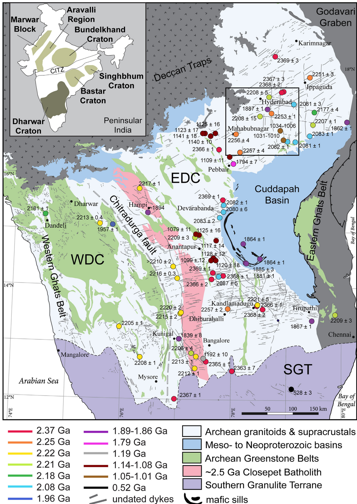
Fig. 1. Generalized geologic map of the Dharwar Craton and study area (black box) modified from Demirel (2012). Major lithologic groupings are represented by pastel colors and U-Pb or Pb-Pb dated Proterozoic dykes are represented by colored circles. EDC: Eastern Dharwar Craton; WDC: Western Dharwar Craton. Top left inset shows the five major cratonic nuclei of Peninsular India, the Marwar Block, and the CITZ.
