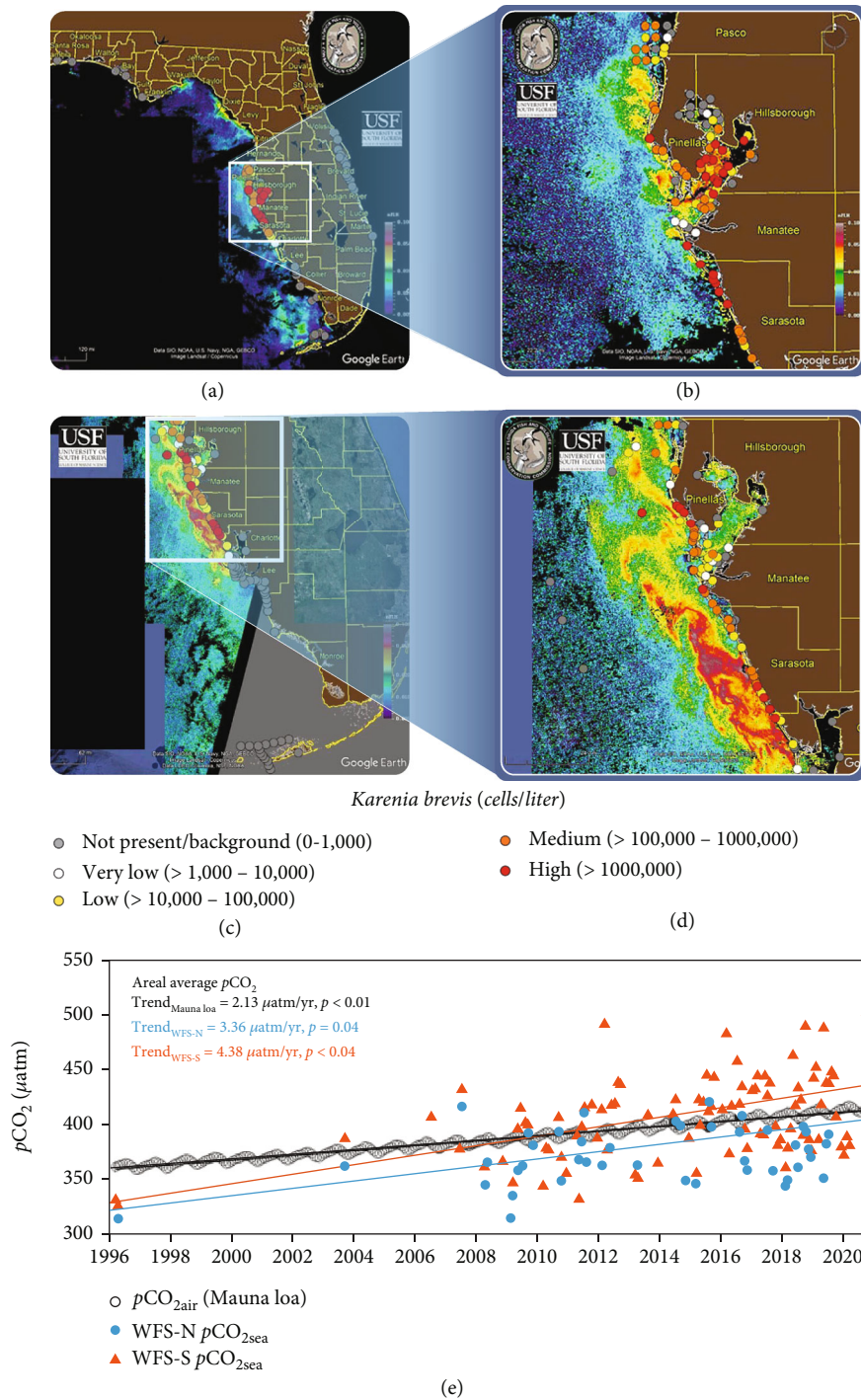
FIGURE 5: Composite of multiple stressors in the West Florida Shelf (WFS). (a, b) Karenia brevis abundance in July 2021 on the West Florida Shelf and regionally in Tampa Bay; (c, d) K. brevis abundance in October 2021 on the southwest Florida Shelf and regionally in Tampa Bay; (e) p\text{CO}_2 increase rates in two subregions of the WFS (north and south) and in the atmosphere. Note that the sea surface p\text{CO}_2 increase rates ( 3.36\text{--}4.38\ \mu\text{atm yr}^{-1} ) in the southern region are much faster than those in the atmosphere ( 2.1\ \mu\text{atm yr}^{-1} ). (a)–(d) are modified from the Florida Fish and Wildlife Research Institute [144], and (e) is from Cai et al. (unpub. data).
