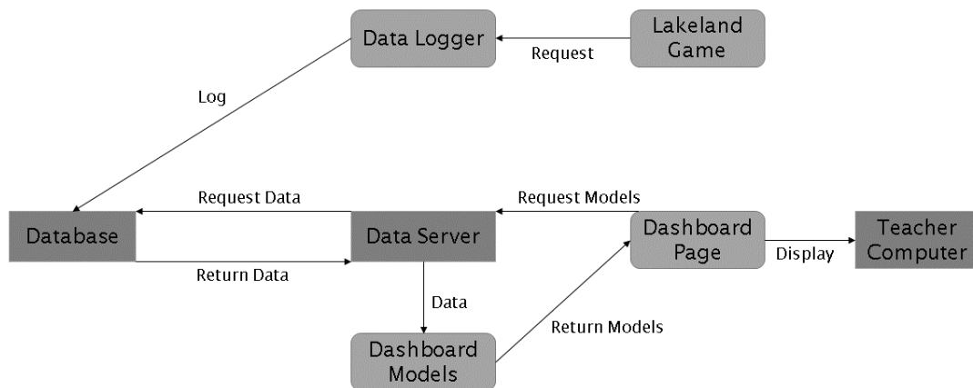
Architecture of Prototype Dashboard Tool
