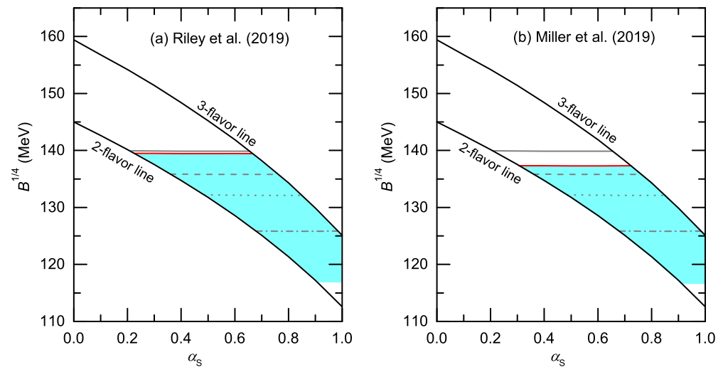
Figure 10. Constraints on the parameters of the standard MIT model for m_s = 93 MeV. The cyan-shadowed areas are the same as those in Figure 2. The gray lines are for \Lambda(1.4) = 580 with f_M = 0, 5\%, 10\% , and 20\% from top to bottom. The red lines also correspond to \Lambda(1.4) = 580 , which are for f_M = 0.5\% in (a) and for f_M = 3.1\% in (b). The image is from [58]. Data from Riley et al. [153] and Miller et al. [154].
